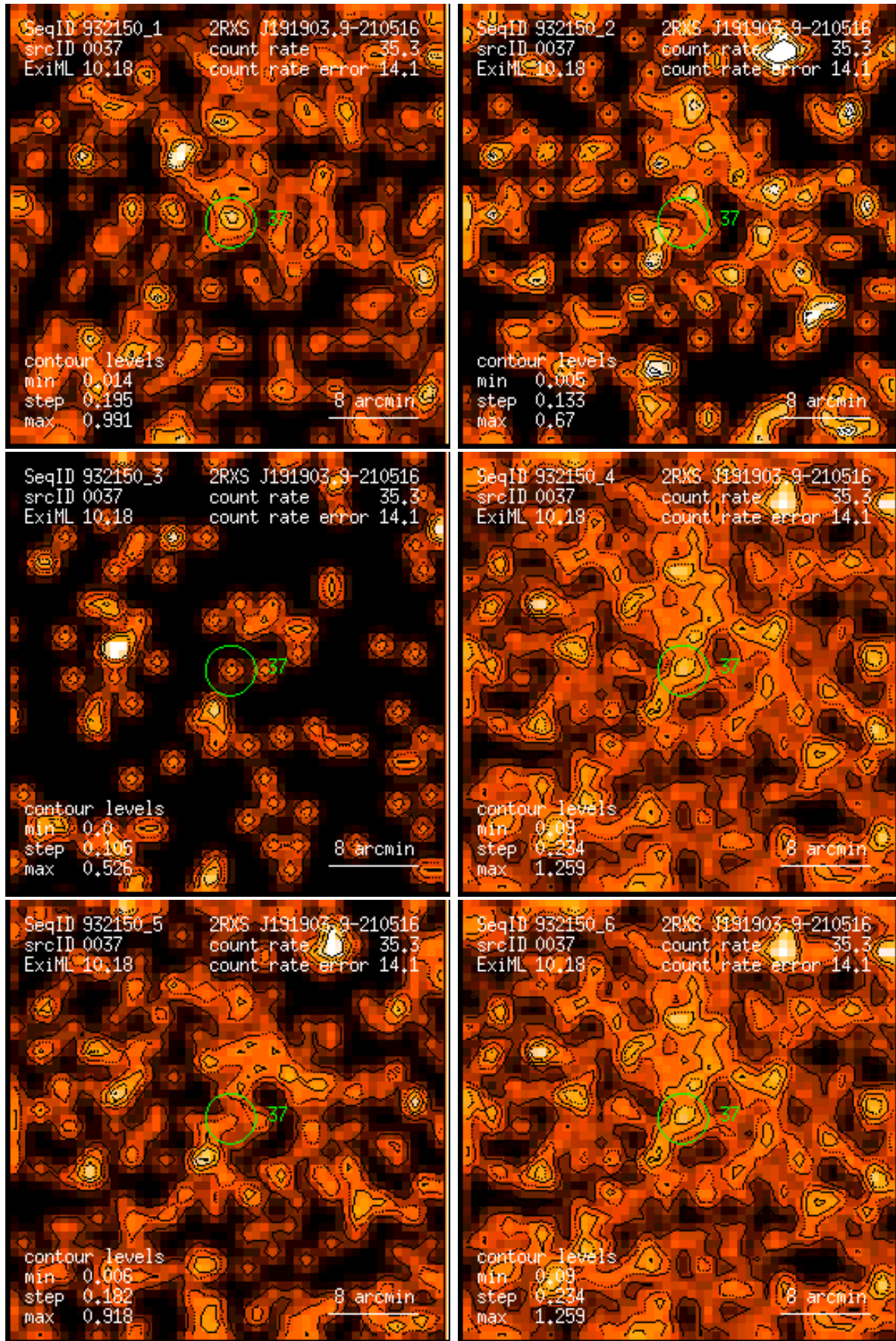
Figure 37: RASS 932150: detection 0037: band rate images, Gaussian filter: (1) PSPC channels 11 – 41, (2) 52 – 90, (3) 91 – 201, (4) 11 – 235, (5) 52 – 201, (6) 11 – 201. Broad band rates in counts/ks. Band rate contour levels in counts/ks/arcmin 2 .
