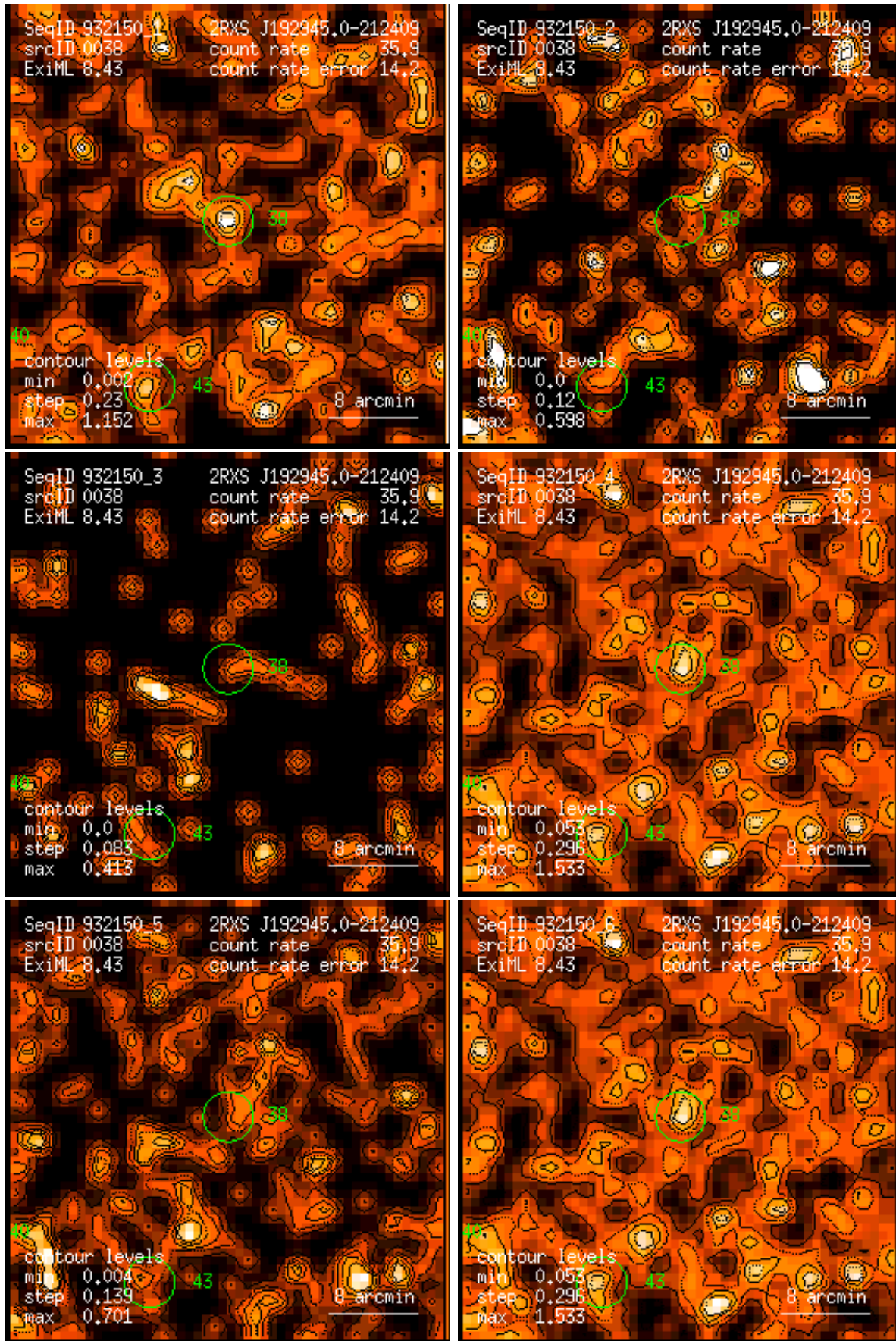
Figure 38: RASS 932150: detection 0038: band rate images, Gaussian filter: (1) PSPC channels 11 – 41, (2) 52 – 90, (3) 91 – 201, (4) 11 – 235, (5) 52 – 201, (6) 11 – 201. Broad band rates in counts/ks. Band rate contour levels in counts/ks/arcmin 2 .
