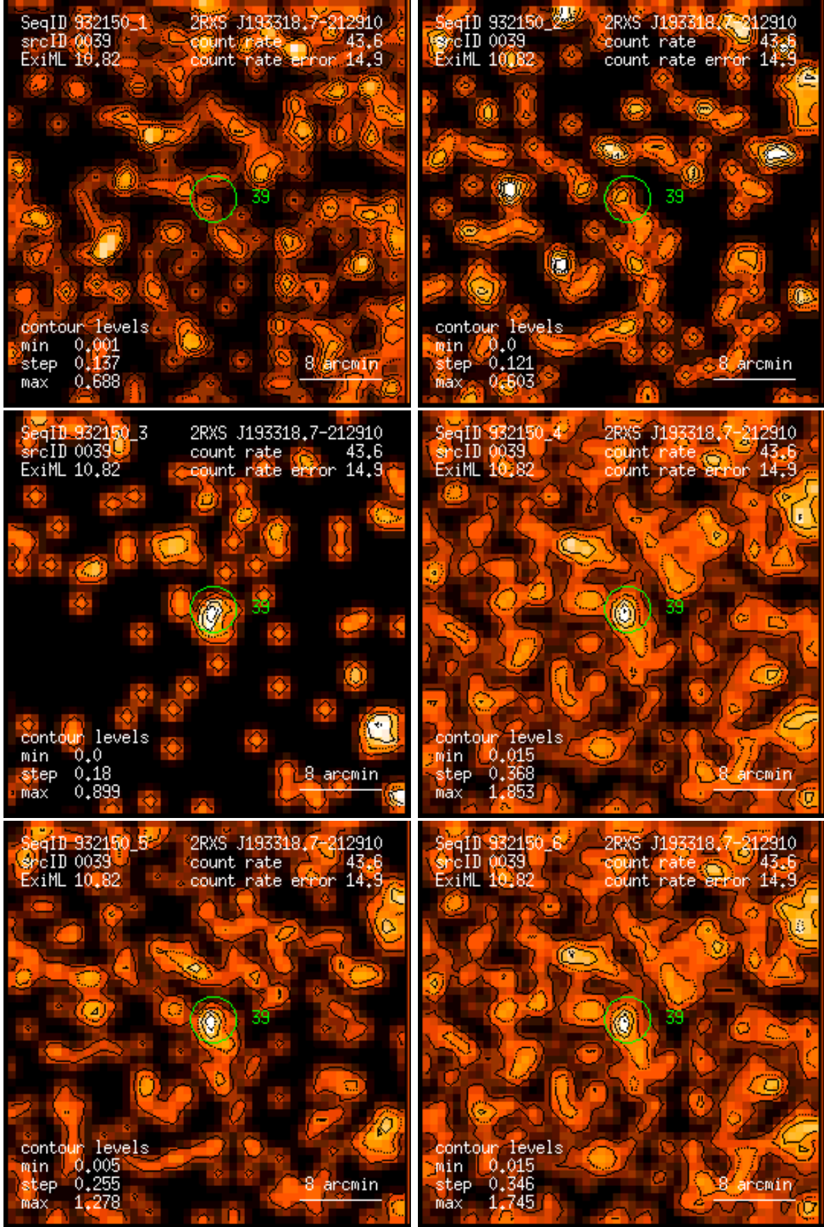
Figure 39: RASS 932150: detection 0039: band rate images, Gaussian filter: (1) PSPC channels 11 – 41, (2) 52 – 90, (3) 91 – 201, (4) 11 – 235, (5) 52 – 201, (6) 11 – 201. Broad band rates in counts/ks. Band rate contour levels in counts/ks/arcmin 2 .
