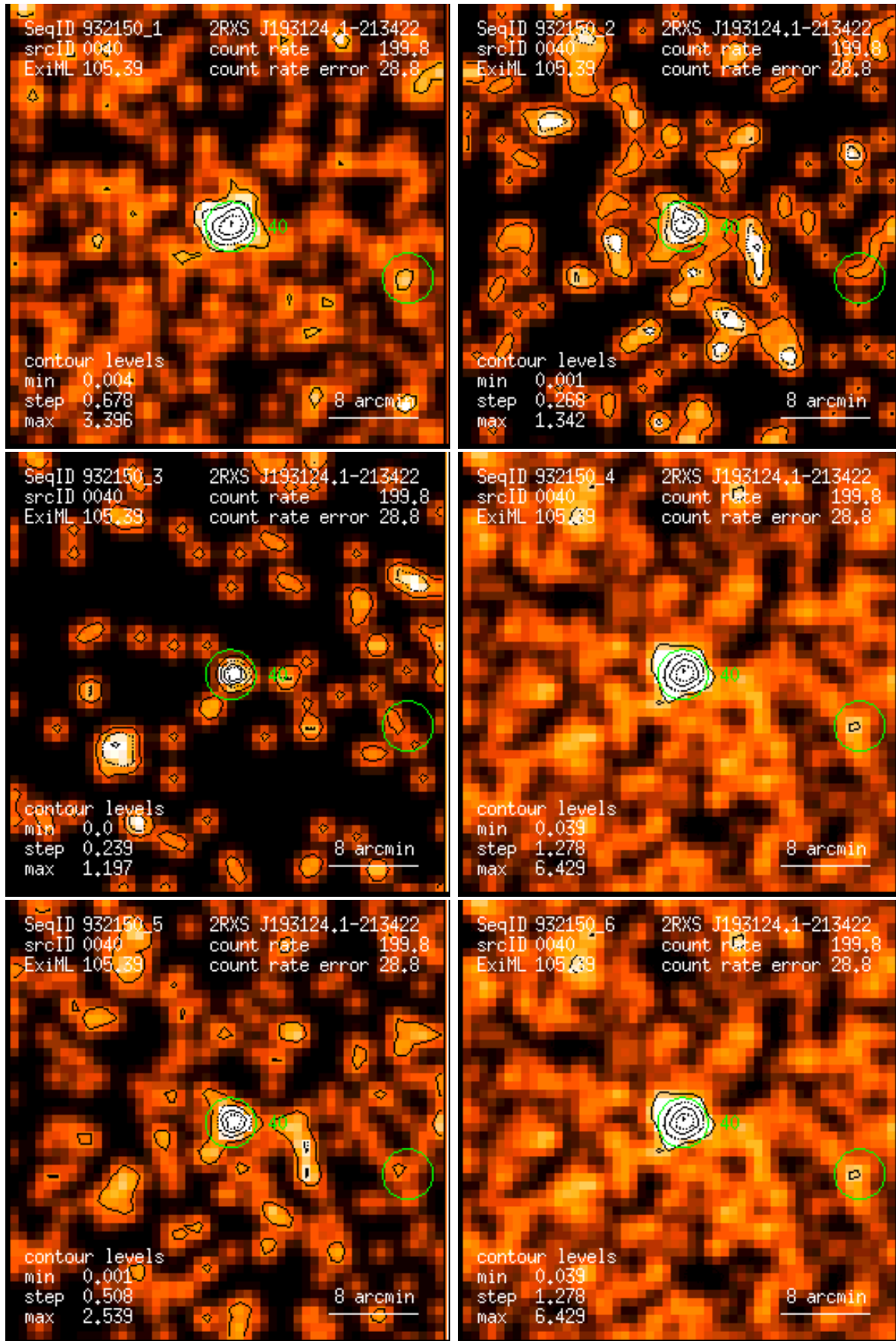
Figure 40: RASS 932150: detection 0040: band rate images, Gaussian filter: (1) PSPC channels 11 – 41, (2) 52 – 90, (3) 91 – 201, (4) 11 – 235, (5) 52 – 201, (6) 11 – 201. Broad band rates in counts/ks. Band rate contour levels in counts/ks/arcmin 2 .
