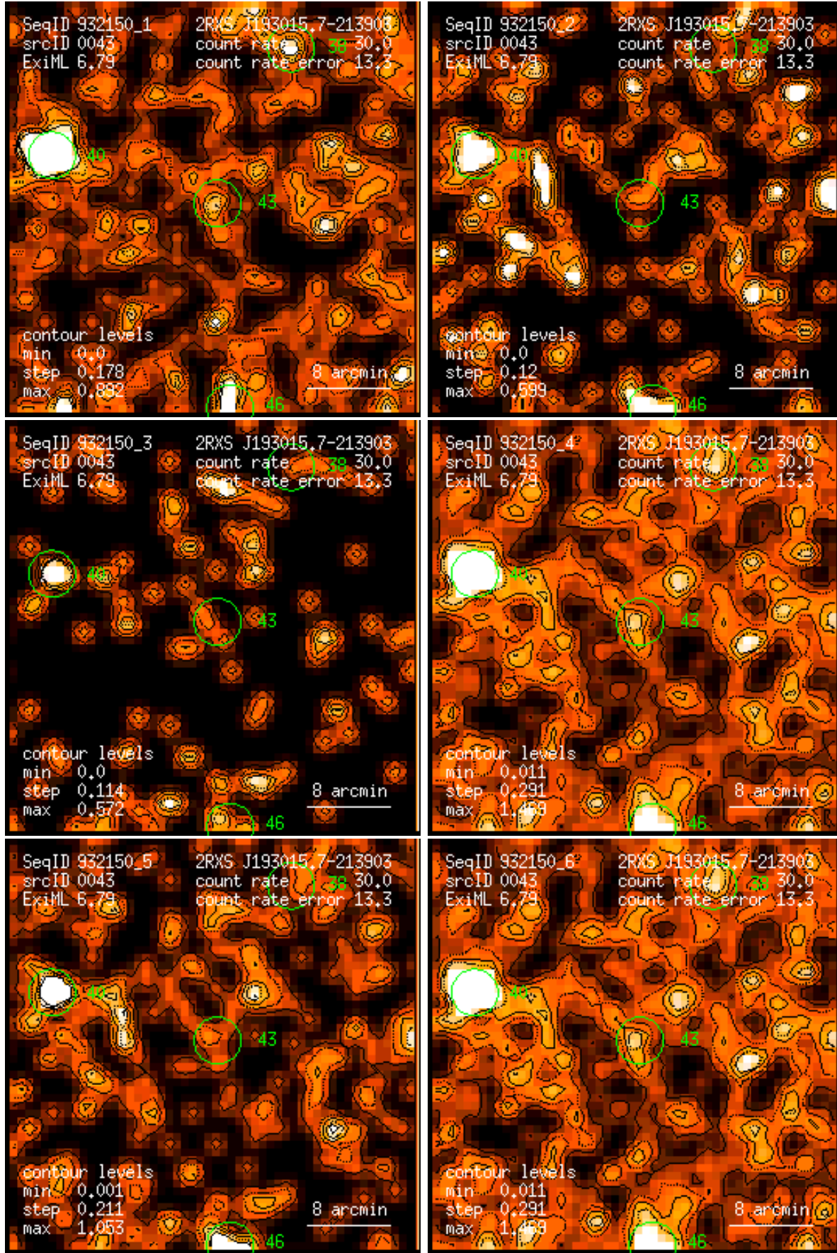
Figure 43: RASS 932150: detection 0043: band rate images, Gaussian filter: (1) PSPC channels 11 – 41, (2) 52 – 90, (3) 91 – 201, (4) 11 – 235, (5) 52 – 201, (6) 11 – 201. Broad band rates in counts/ks. Band rate contour levels in counts/ks/arcmin 2 .
