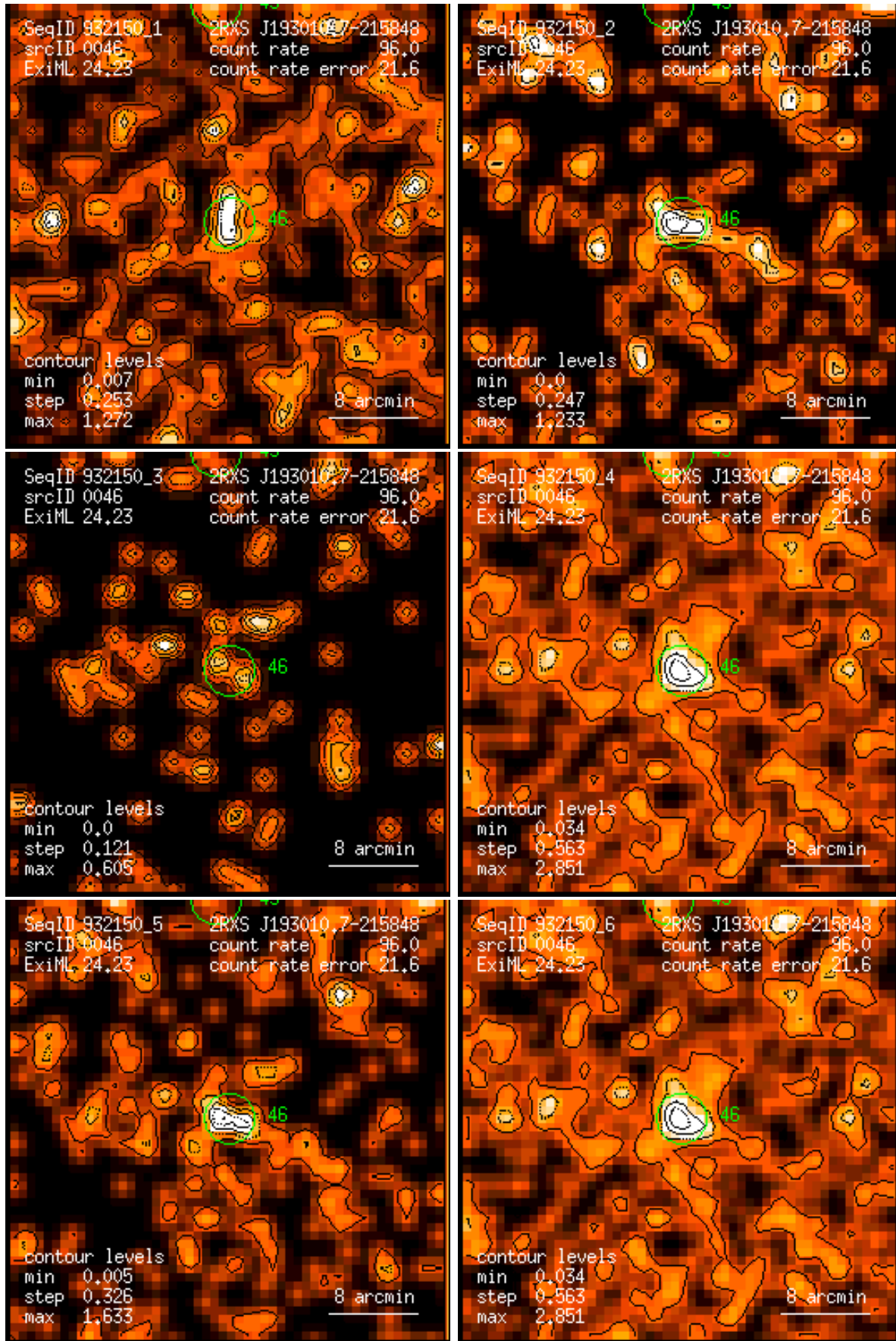
Figure 46: RASS 932150: detection 0046: band rate images, Gaussian filter: (1) PSPC channels 11 – 41, (2) 52 – 90, (3) 91 – 201, (4) 11 – 235, (5) 52 – 201, (6) 11 – 201. Broad band rates in counts/ks. Band rate contour levels in counts/ks/arcmin 2 .
