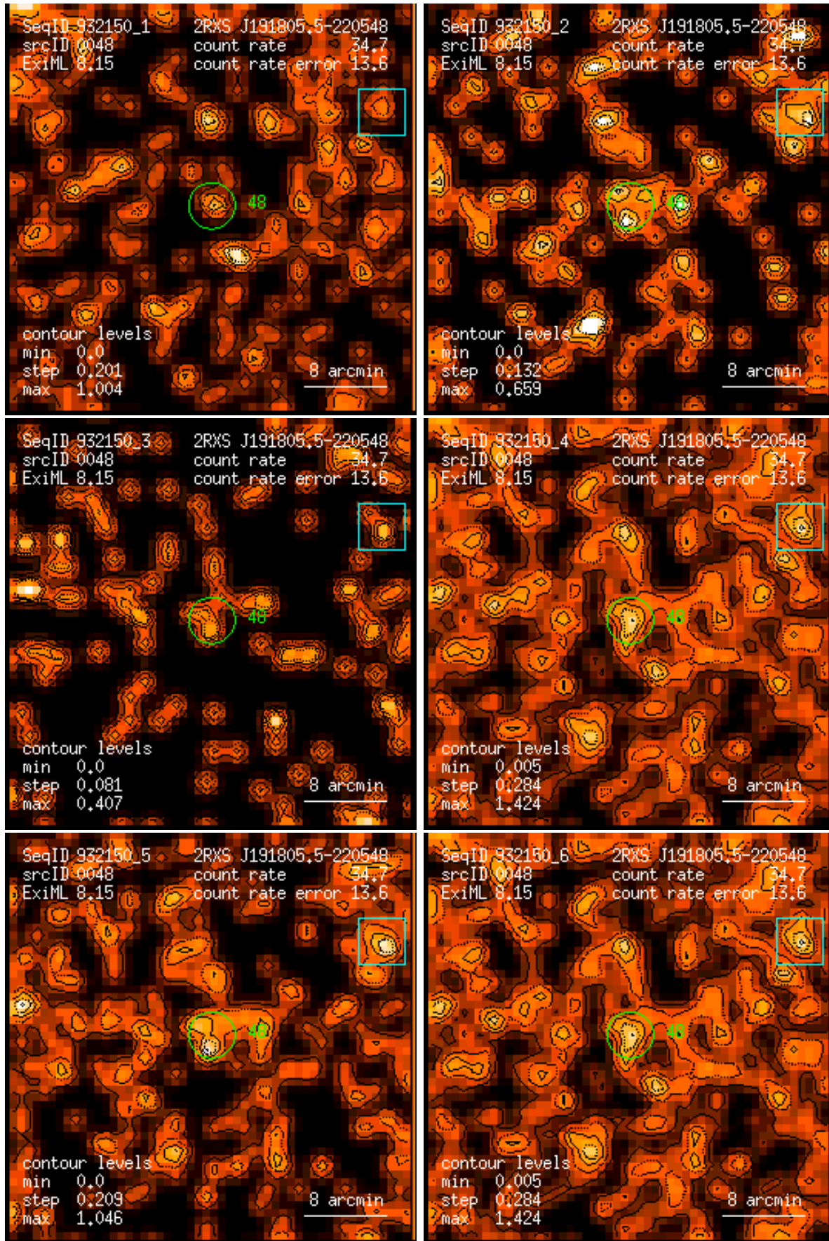
Figure 48: RASS 932150: detection 0048: band rate images, Gaussian filter: (1) PSPC channels 11 – 41, (2) 52 – 90, (3) 91 – 201, (4) 11 – 235, (5) 52 – 201, (6) 11 – 201. Broad band rates in counts/ks. Band rate contour levels in counts/ks/arcmin 2 .
