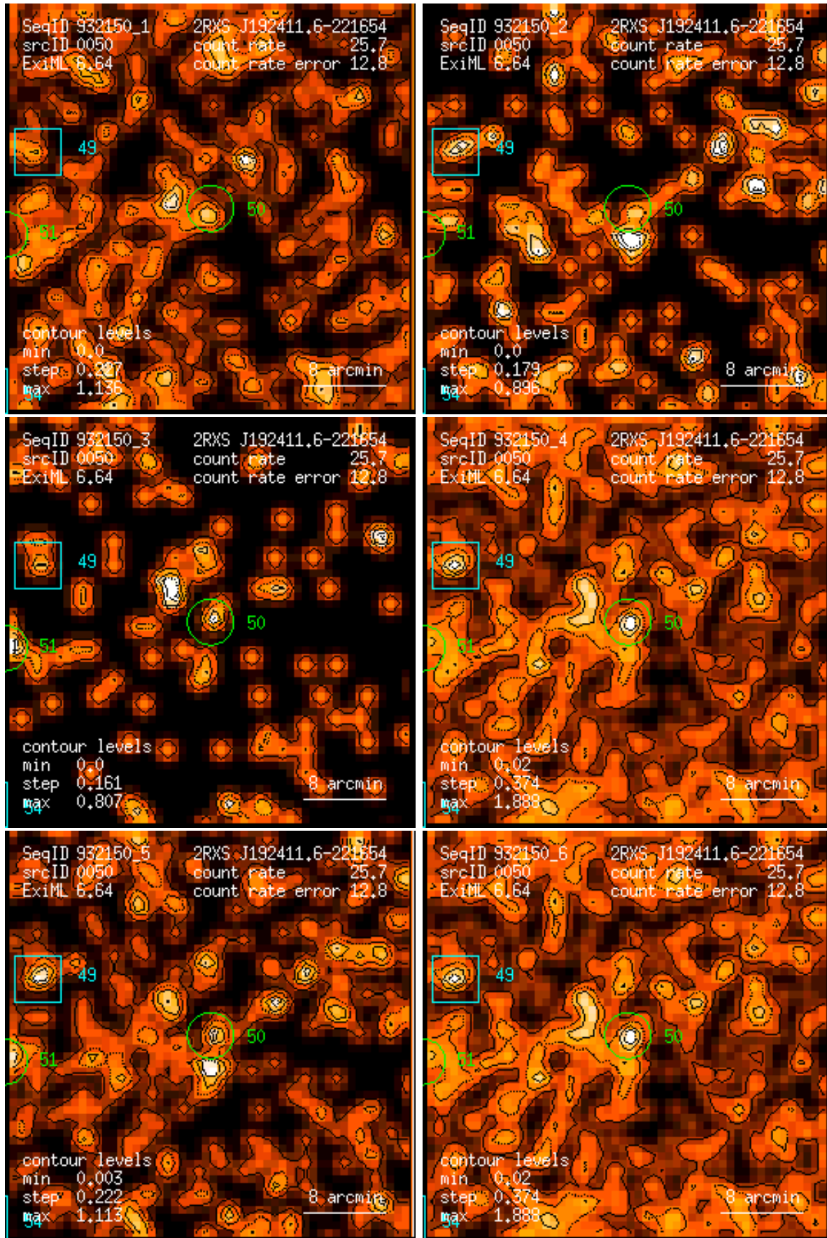
Figure 50: RASS 932150: detection 0050: band rate images, Gaussian filter: (1) PSPC channels 11 – 41, (2) 52 – 90, (3) 91 – 201, (4) 11 – 235, (5) 52 – 201, (6) 11 – 201. Broad band rates in counts/ks. Band rate contour levels in counts/ks/arcmin 2 .
