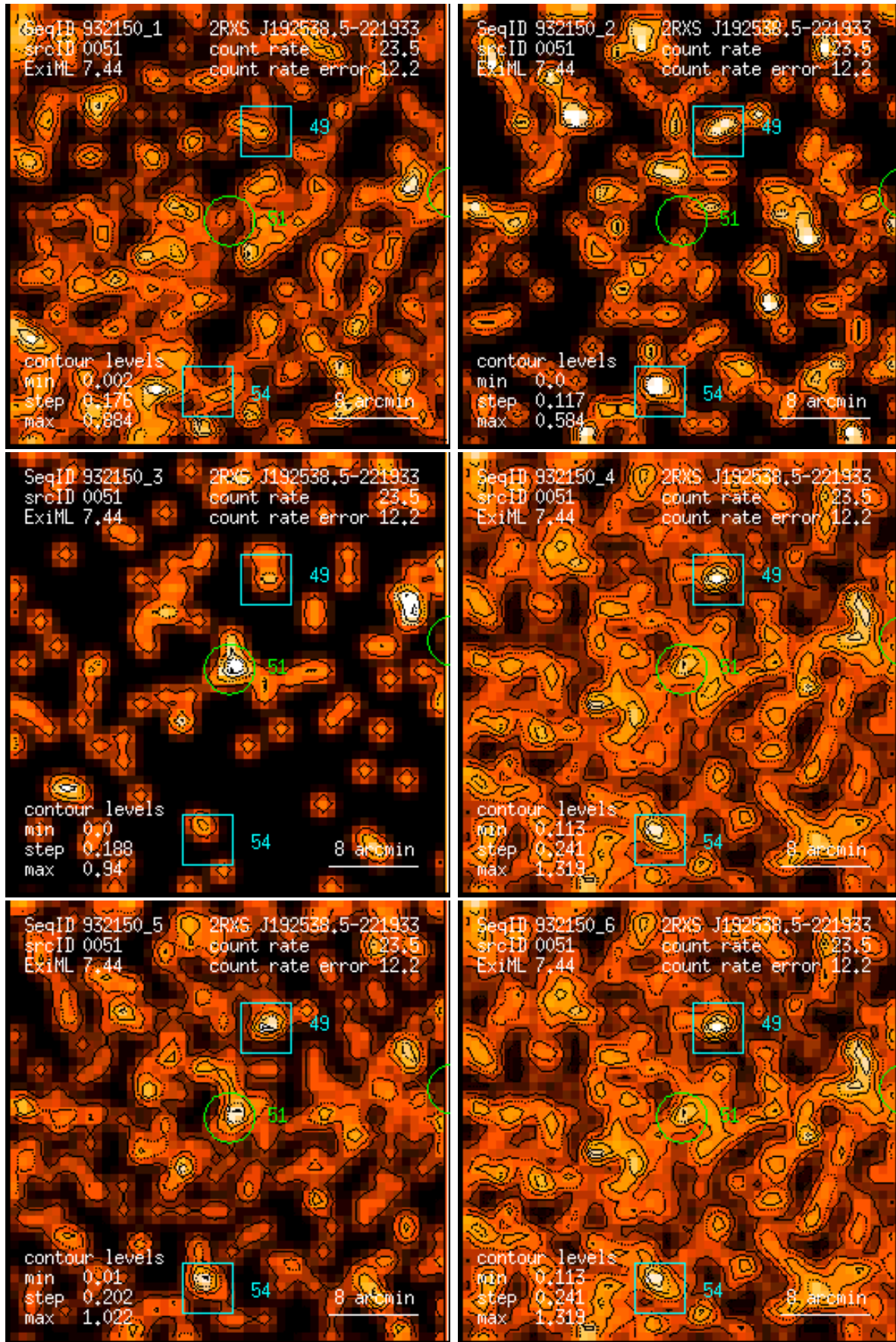
Figure 51: RASS 932150: detection 0051: band rate images, Gaussian filter: (1) PSPC channels 11 – 41, (2) 52 – 90, (3) 91 – 201, (4) 11 – 235, (5) 52 – 201, (6) 11 – 201. Broad band rates in counts/ks. Band rate contour levels in counts/ks/arcmin 2 .
