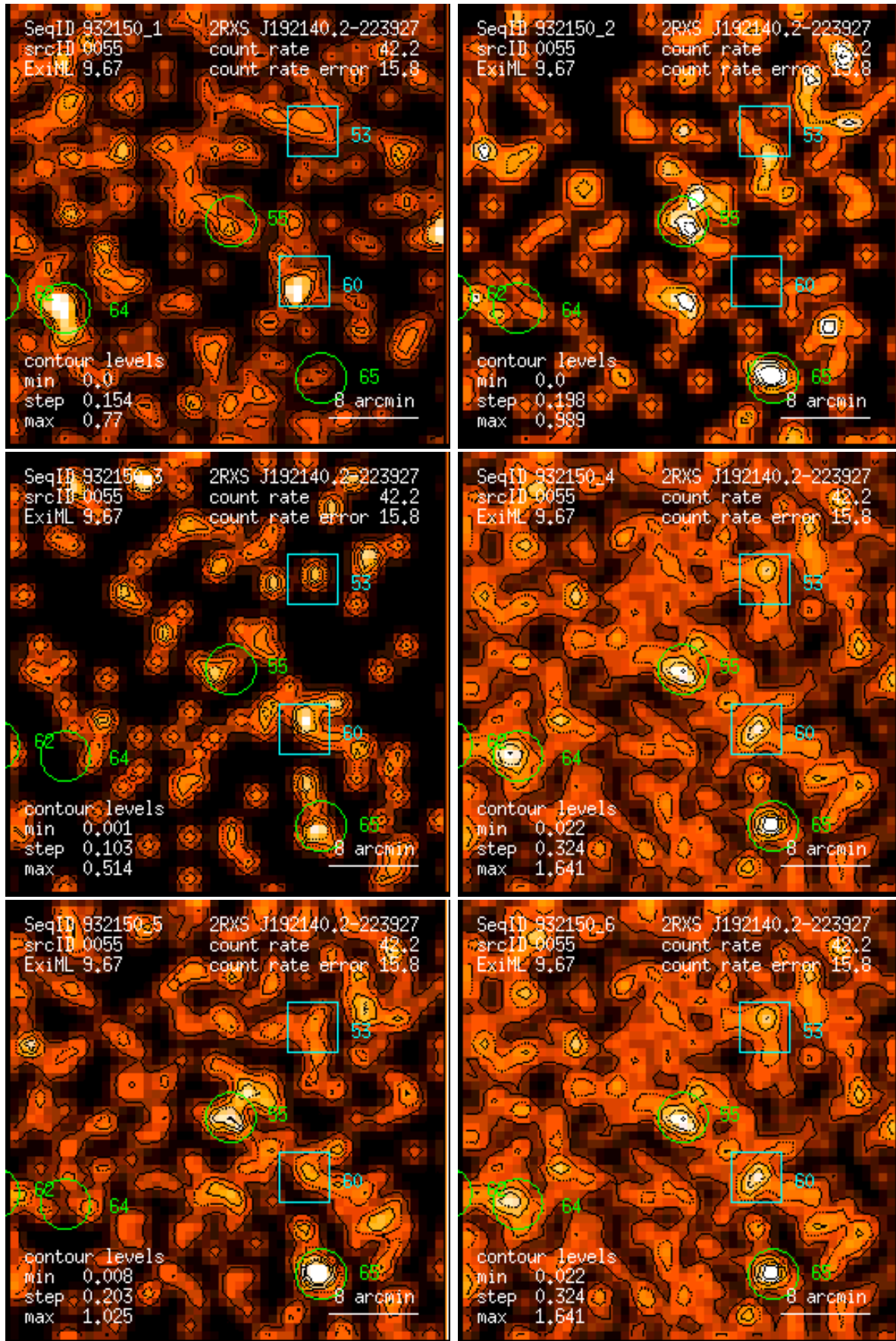
Figure 55: RASS 932150: detection 0055: band rate images, Gaussian filter: (1) PSPC channels 11 – 41, (2) 52 – 90, (3) 91 – 201, (4) 11 – 235, (5) 52 – 201, (6) 11 – 201. Broad band rates in counts/ks. Band rate contour levels in counts/ks/arcmin 2 .
