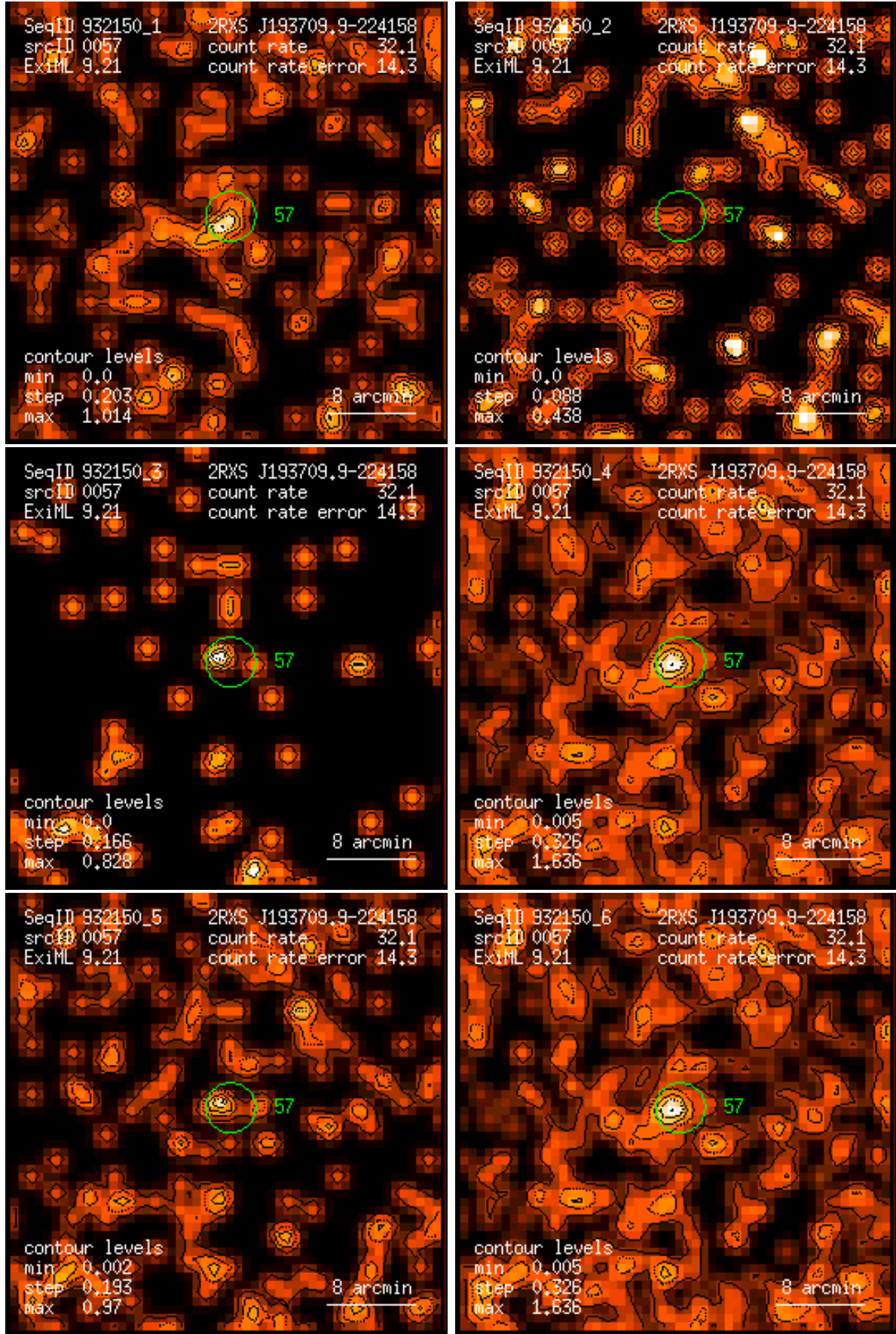
Figure 57: RASS 932150: detection 0057: band rate images, Gaussian filter: (1) PSPC channels 11 – 41, (2) 52 – 90, (3) 91 – 201, (4) 11 – 235, (5) 52 – 201, (6) 11 – 201. Broad band rates in counts/ks. Band rate contour levels in counts/ks/arcmin 2 .
