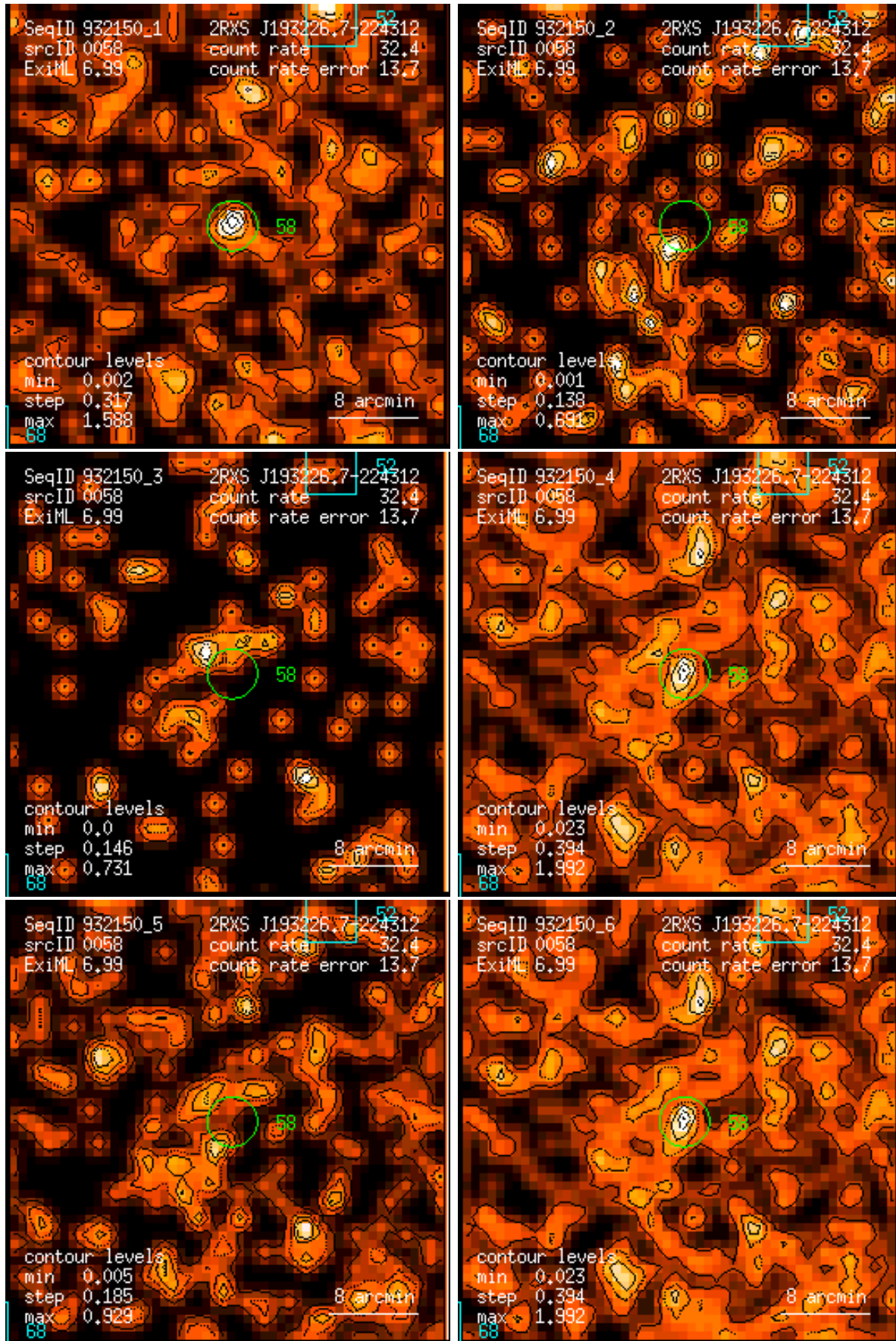
Figure 58: RASS 932150: detection 0058: band rate images, Gaussian filter: (1) PSPC channels 11 – 41, (2) 52 – 90, (3) 91 – 201, (4) 11 – 235, (5) 52 – 201, (6) 11 – 201. Broad band rates in counts/ks. Band rate contour levels in counts/ks/arcmin 2 .
