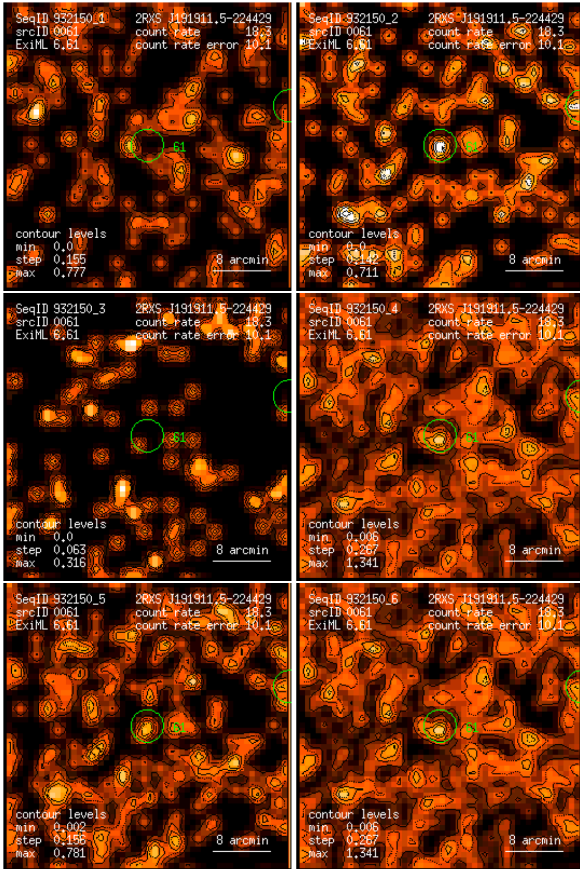
Figure 61: RASS 932150: detection 0061: band rate images, Gaussian filter: (1) PSPC channels 11 – 41, (2) 52 – 90, (3) 91 – 201, (4) 11 – 235, (5) 52 – 201, (6) 11 – 201. Broad band rates in counts/ks. Band rate contour levels in counts/ks/arcmin 2 .
