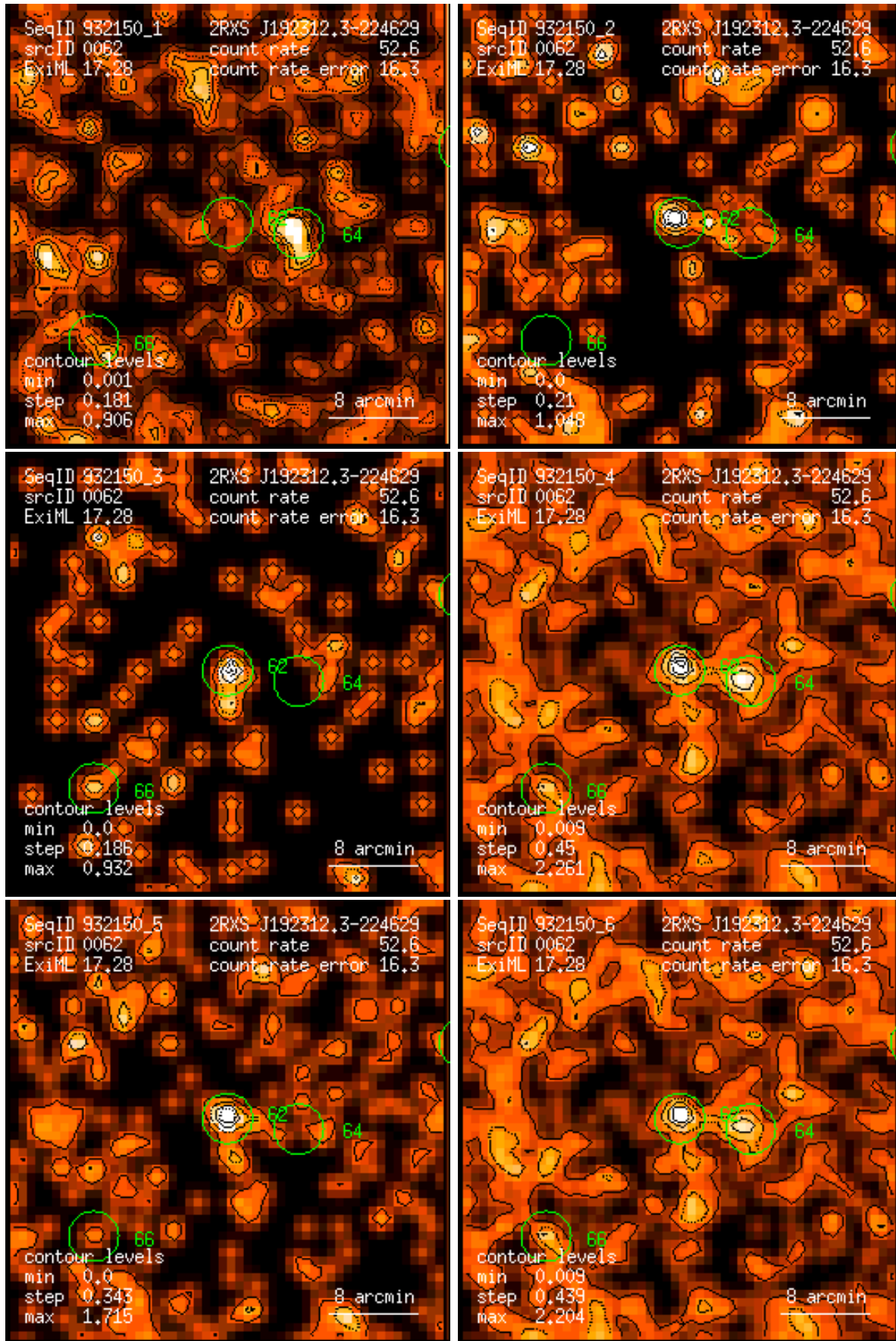
Figure 62: RASS 932150: detection 0062: band rate images, Gaussian filter: (1) PSPC channels 11 – 41, (2) 52 – 90, (3) 91 – 201, (4) 11 – 235, (5) 52 – 201, (6) 11 – 201. Broad band rates in counts/ks. Band rate contour levels in counts/ks/arcmin 2 .
