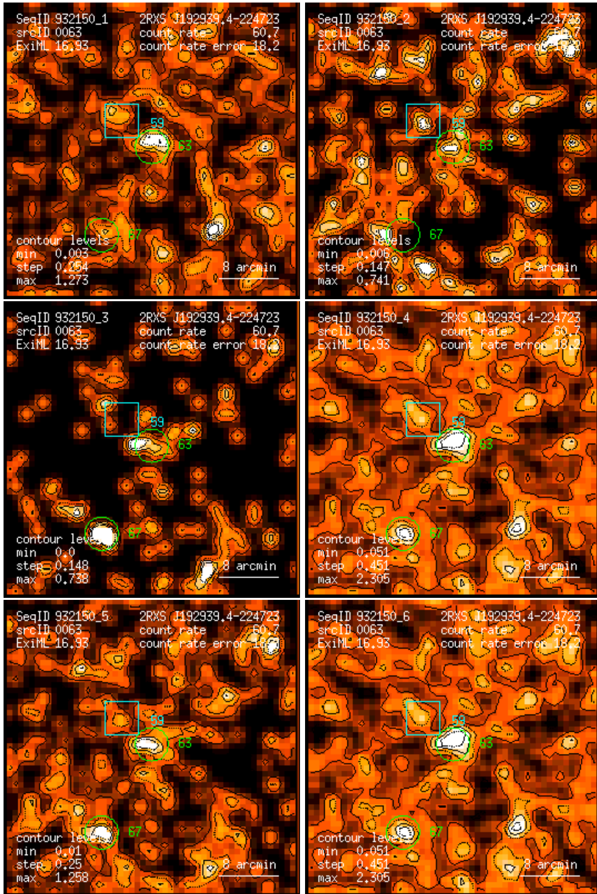
Figure 63: RASS 932150: detection 0063: band rate images, Gaussian filter: (1) PSPC channels 11 – 41, (2) 52 – 90, (3) 91 – 201, (4) 11 – 235, (5) 52 – 201, (6) 11 – 201. Broad band rates in counts/ks. Band rate contour levels in counts/ks/arcmin 2 .
