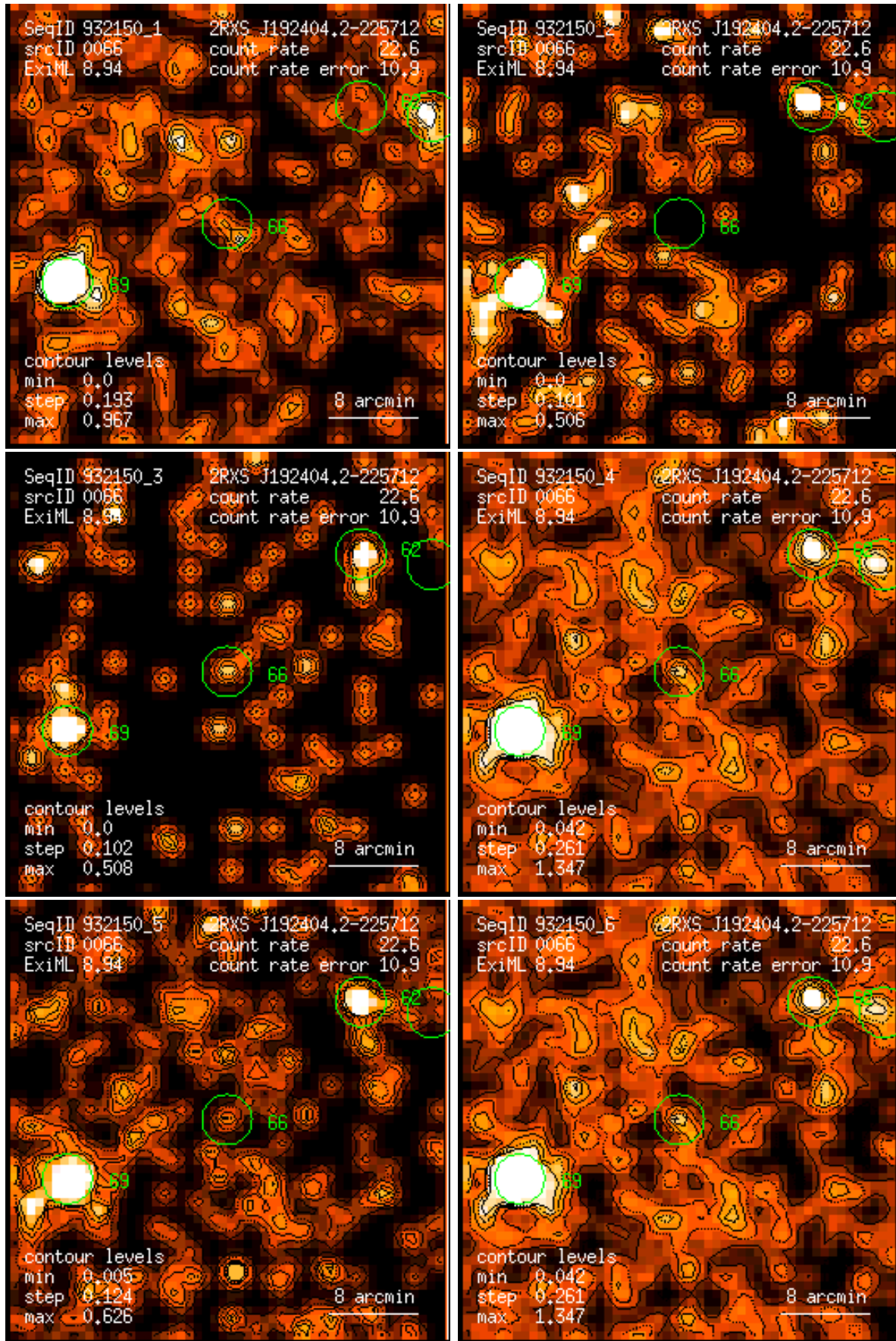
Figure 66: RASS 932150: detection 0066: band rate images, Gaussian filter: (1) PSPC channels 11 – 41, (2) 52 – 90, (3) 91 – 201, (4) 11 – 235, (5) 52 – 201, (6) 11 – 201. Broad band rates in counts/ks. Band rate contour levels in counts/ks/arcmin 2 .
