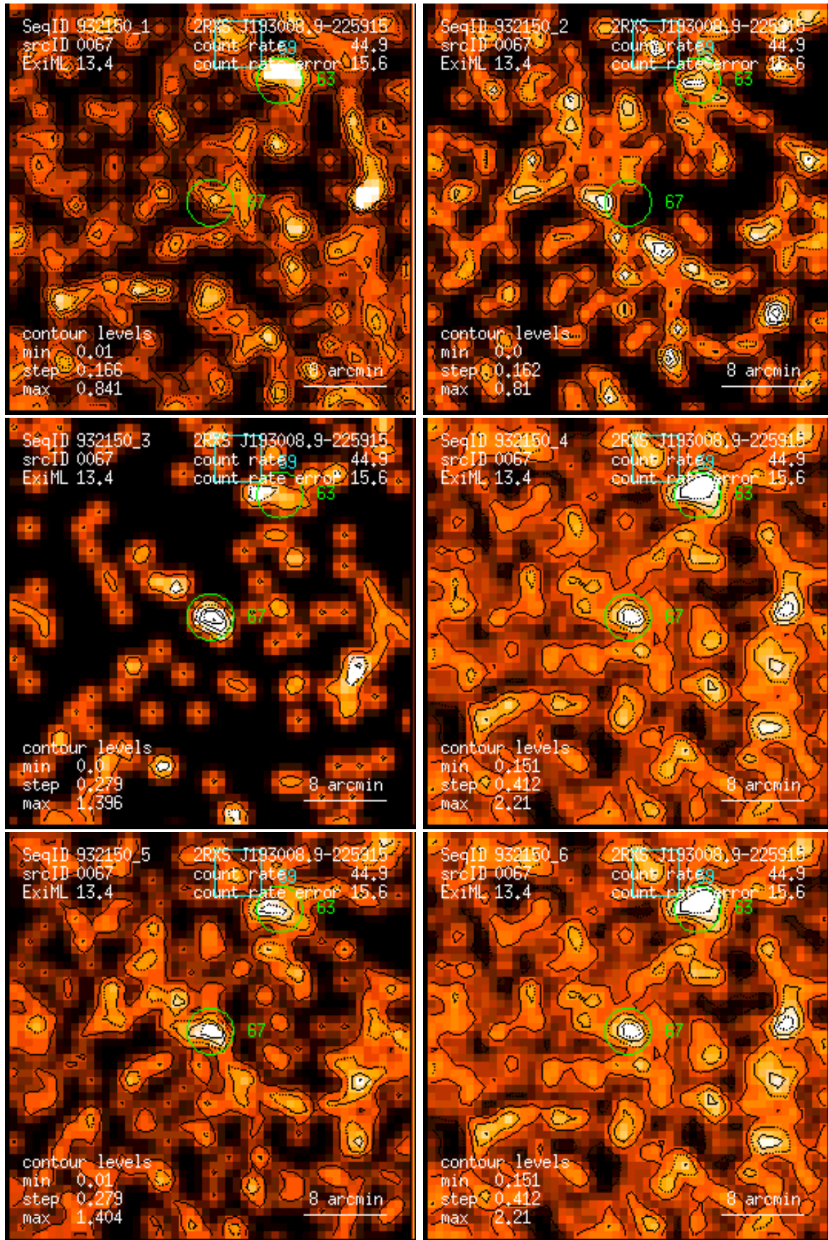
Figure 67: RASS 932150: detection 0067: band rate images, Gaussian filter: (1) PSPC channels 11 – 41, (2) 52 – 90, (3) 91 – 201, (4) 11 – 235, (5) 52 – 201, (6) 11 – 201. Broad band rates in counts/ks. Band rate contour levels in counts/ks/arcmin 2 .
