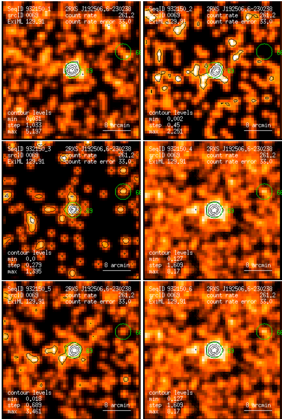
Figure 69: RASS 932150: detection 0069: band rate images, Gaussian filter: (1) PSPC channels 11 – 41, (2) 52 – 90, (3) 91 – 201, (4) 11 – 235, (5) 52 – 201, (6) 11 – 201. Broad band rates in counts/ks. Band rate contour levels in counts/ks/arcmin 2 .
