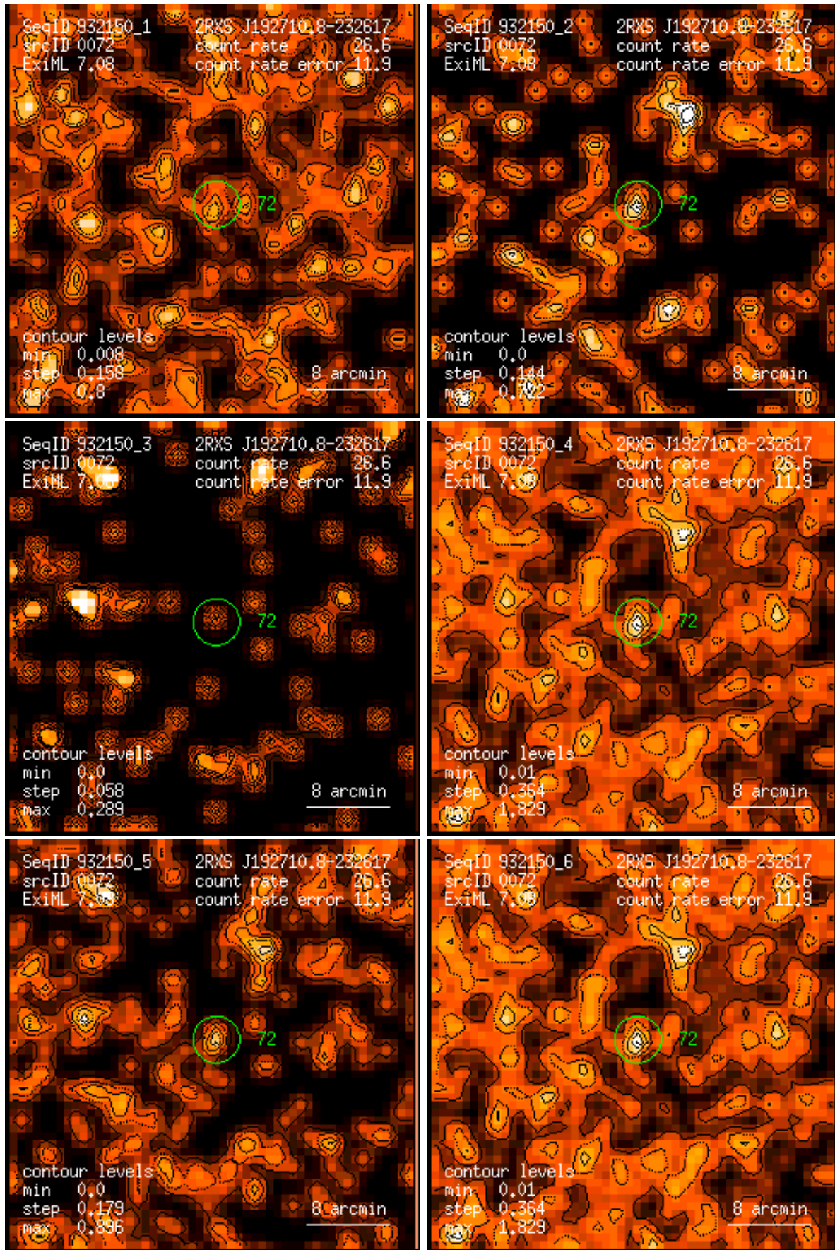
Figure 72: RASS 932150: detection 0072: band rate images, Gaussian filter: (1) PSPC channels 11 – 41, (2) 52 – 90, (3) 91 – 201, (4) 11 – 235, (5) 52 – 201, (6) 11 – 201. Broad band rates in counts/ks. Band rate contour levels in counts/ks/arcmin 2 .
