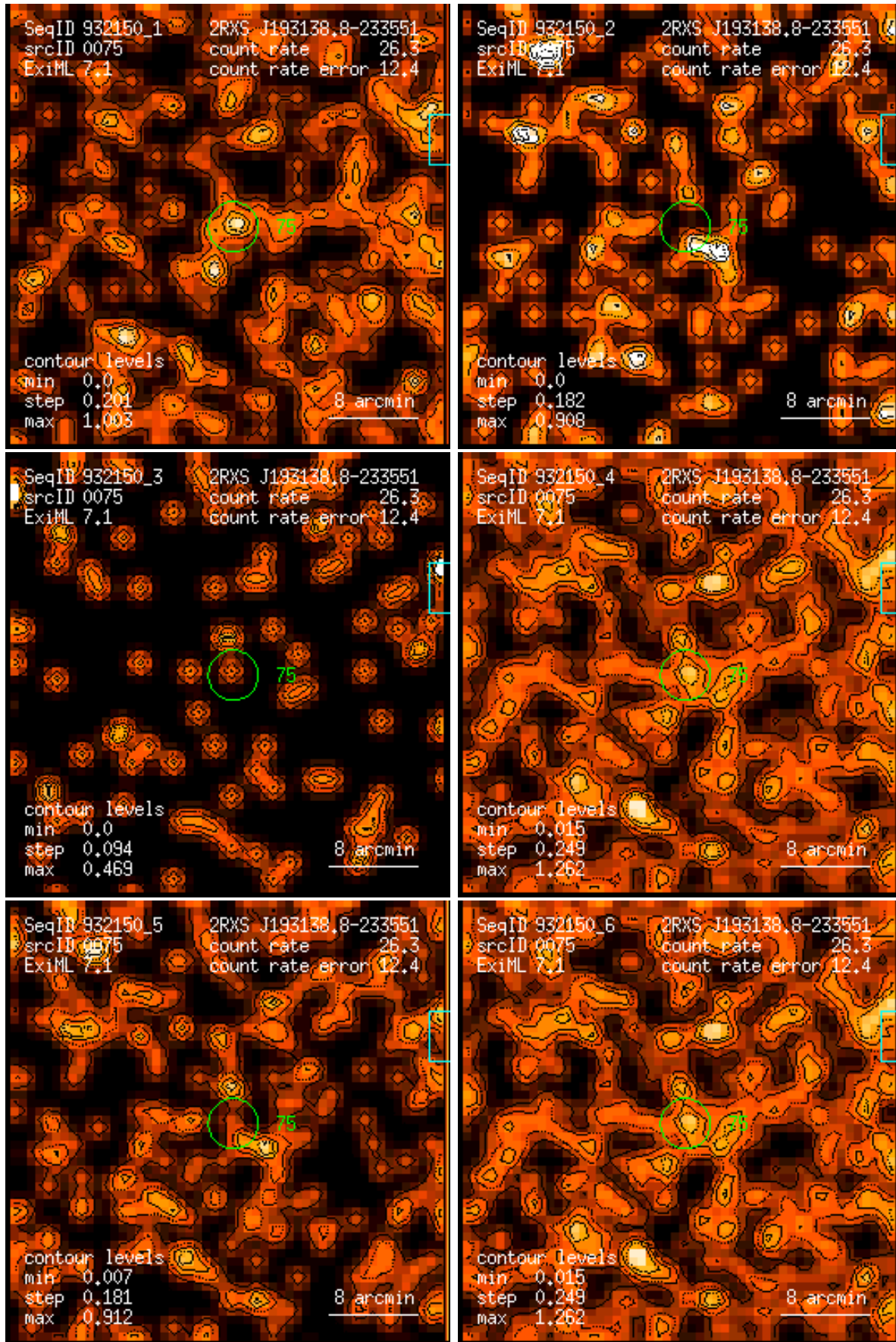
Figure 75: RASS 932150: detection 0075: band rate images, Gaussian filter: (1) PSPC channels 11 – 41, (2) 52 – 90, (3) 91 – 201, (4) 11 – 235, (5) 52 – 201, (6) 11 – 201. Broad band rates in counts/ks. Band rate contour levels in counts/ks/arcmin 2 .
