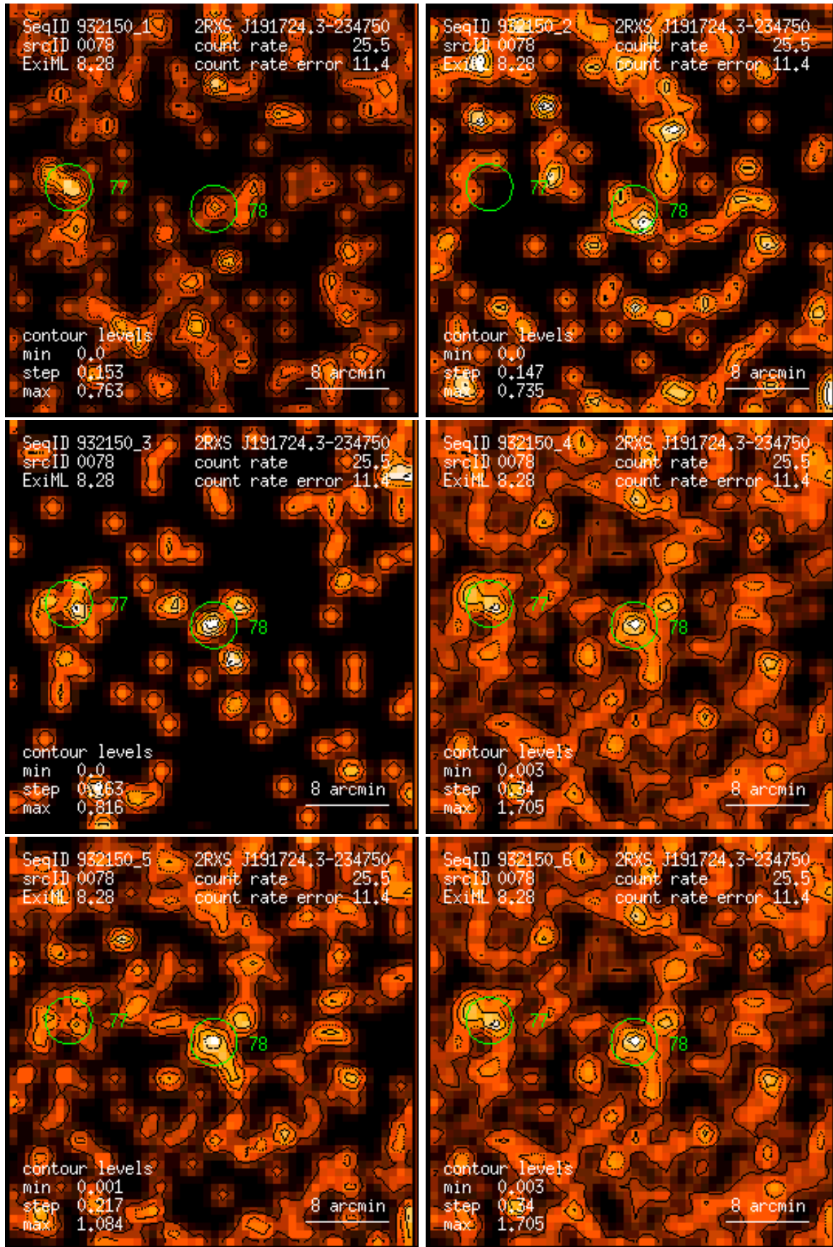
Figure 78: RASS 932150: detection 0078: band rate images, Gaussian filter: (1) PSPC channels 11 – 41, (2) 52 – 90, (3) 91 – 201, (4) 11 – 235, (5) 52 – 201, (6) 11 – 201. Broad band rates in counts/ks. Band rate contour levels in counts/ks/arcmin 2 .
