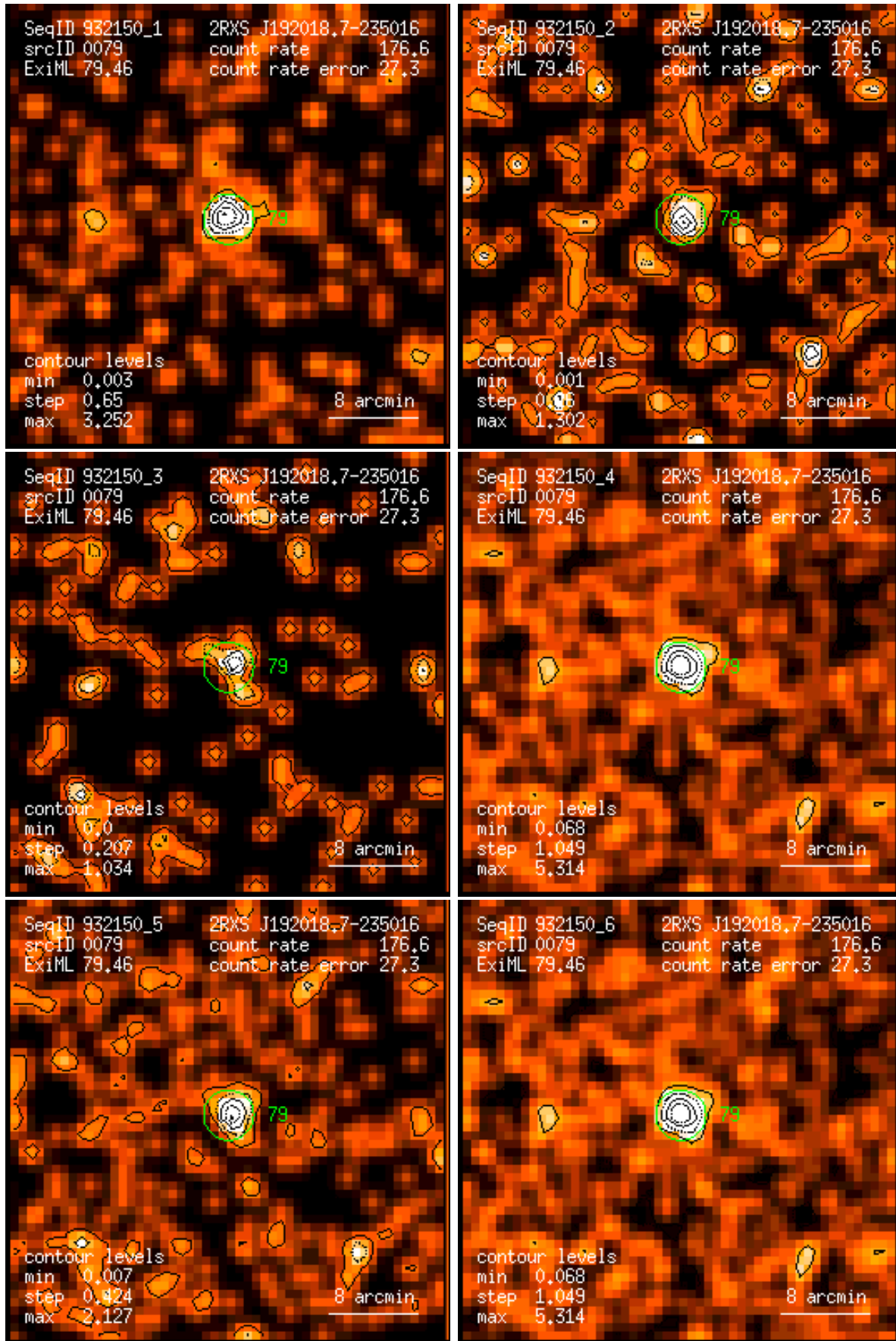
Figure 79: RASS 932150: detection 0079: band rate images, Gaussian filter: (1) PSPC channels 11 – 41, (2) 52 – 90, (3) 91 – 201, (4) 11 – 235, (5) 52 – 201, (6) 11 – 201. Broad band rates in counts/ks. Band rate contour levels in counts/ks/arcmin 2 .
