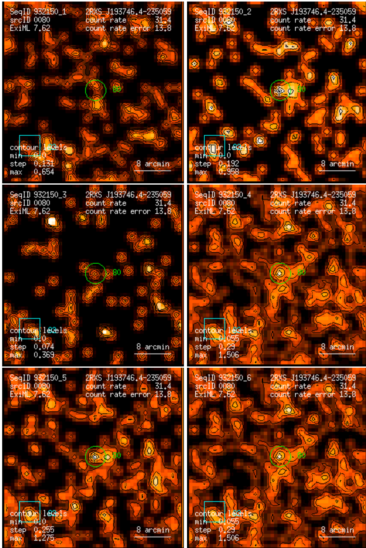
Figure 80: RASS 932150: detection 0080: band rate images, Gaussian filter: (1) PSPC channels 11 – 41, (2) 52 – 90, (3) 91 – 201, (4) 11 – 235, (5) 52 – 201, (6) 11 – 201. Broad band rates in counts/ks. Band rate contour levels in counts/ks/arcmin 2 .
