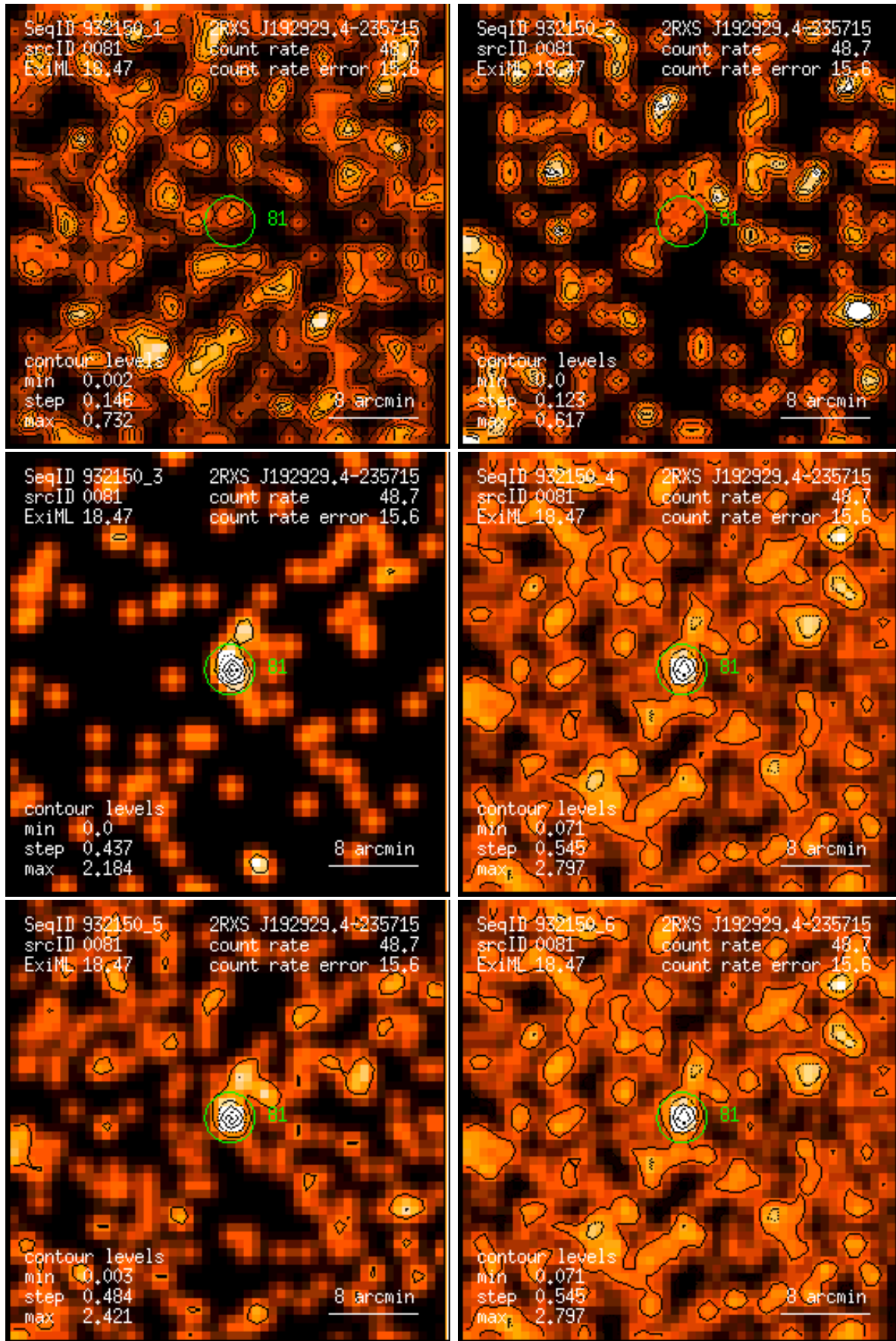
Figure 81: RASS 932150: detection 0081: band rate images, Gaussian filter: (1) PSPC channels 11 – 41, (2) 52 – 90, (3) 91 – 201, (4) 11 – 235, (5) 52 – 201, (6) 11 – 201. Broad band rates in counts/ks. Band rate contour levels in counts/ks/arcmin 2 .
