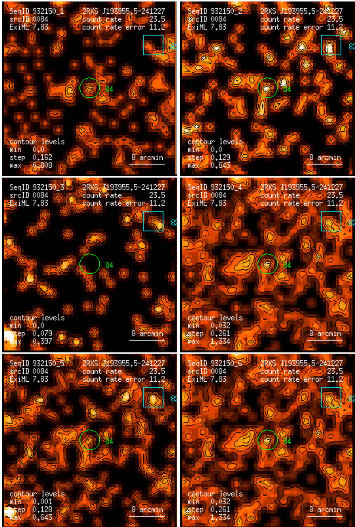
Figure 84: RASS 932150: detection 0084: band rate images, Gaussian filter: (1) PSPC channels 11 – 41, (2) 52 – 90, (3) 91 – 201, (4) 11 – 235, (5) 52 – 201, (6) 11 – 201. Broad band rates in counts/ks. Band rate contour levels in counts/ks/arcmin 2 .
