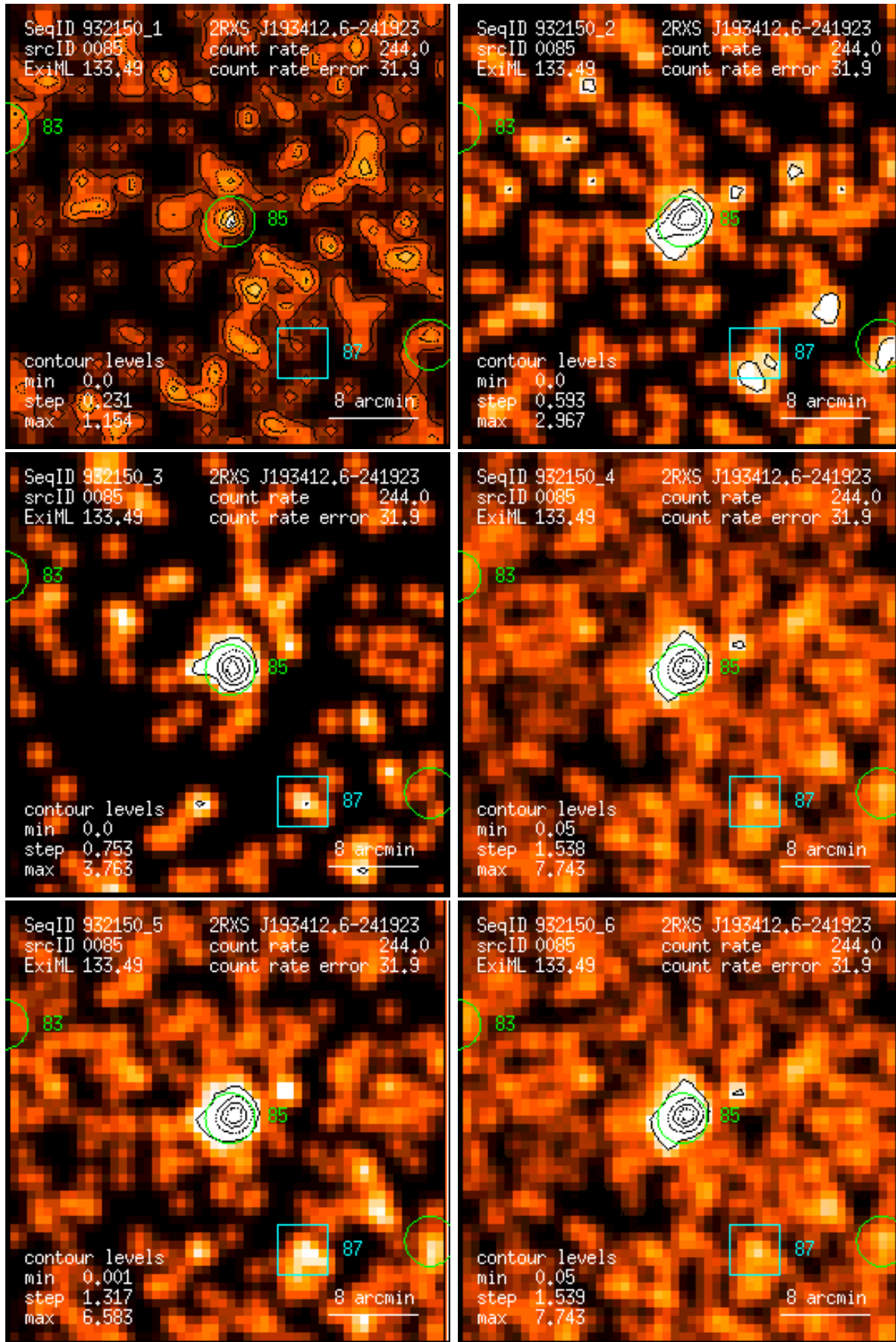
Figure 85: RASS 932150: detection 0085: band rate images, Gaussian filter: (1) PSPC channels 11 – 41, (2) 52 – 90, (3) 91 – 201, (4) 11 – 235, (5) 52 – 201, (6) 11 – 201. Broad band rates in counts/ks. Band rate contour levels in counts/ks/arcmin 2 .
