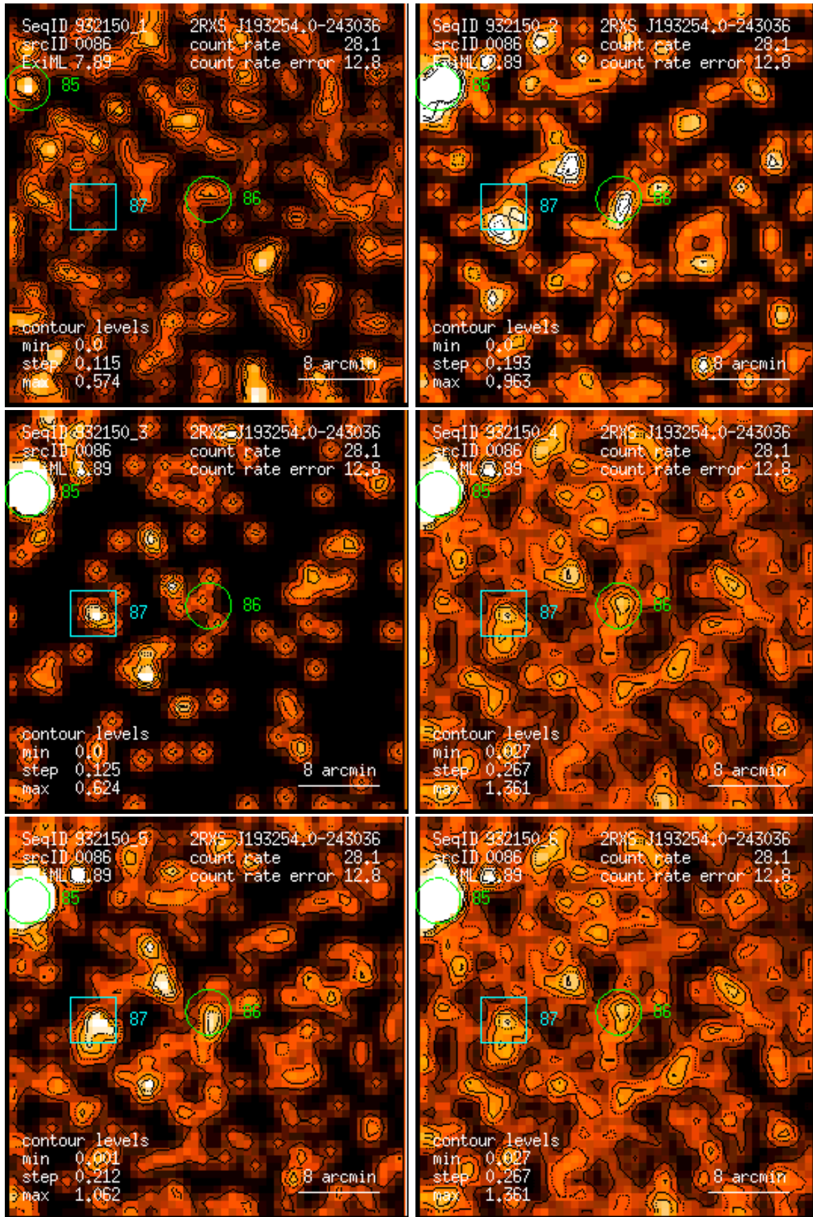
Figure 86: RASS 932150: detection 0086: band rate images, Gaussian filter: (1) PSPC channels 11 – 41, (2) 52 – 90, (3) 91 – 201, (4) 11 – 235, (5) 52 – 201, (6) 11 – 201. Broad band rates in counts/ks. Band rate contour levels in counts/ks/arcmin 2 .
