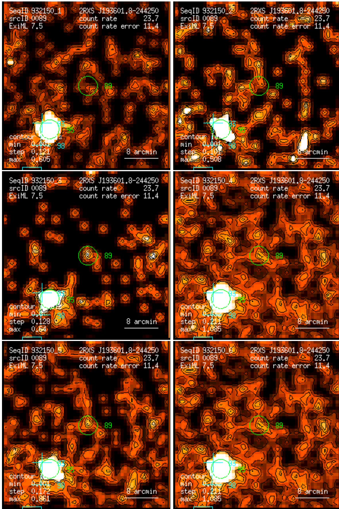
Figure 89: RASS 932150: detection 0089: band rate images, Gaussian filter: (1) PSPC channels 11 – 41, (2) 52 – 90, (3) 91 – 201, (4) 11 – 235, (5) 52 – 201, (6) 11 – 201. Broad band rates in counts/ks. Band rate contour levels in counts/ks/arcmin 2 .
