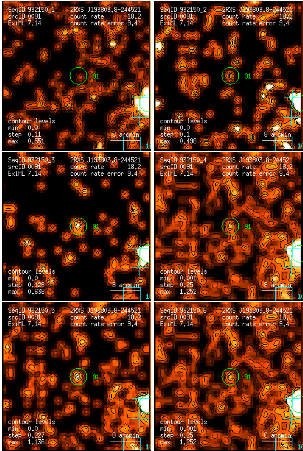
Figure 91: RASS 932150: detection 0091: band rate images, Gaussian filter: (1) PSPC channels 11 – 41, (2) 52 – 90, (3) 91 – 201, (4) 11 – 235, (5) 52 – 201, (6) 11 – 201. Broad band rates in counts/ks. Band rate contour levels in counts/ks/arcmin 2 .
