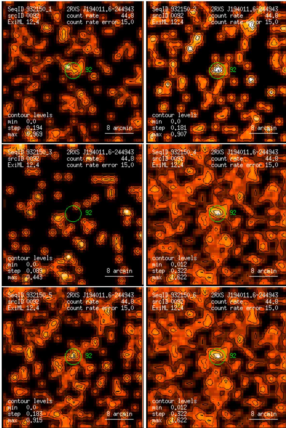
Figure 92: RASS 932150: detection 0092: band rate images, Gaussian filter: (1) PSPC channels 11 – 41, (2) 52 – 90, (3) 91 – 201, (4) 11 – 235, (5) 52 – 201, (6) 11 – 201. Broad band rates in counts/ks. Band rate contour levels in counts/ks/arcmin 2 .
