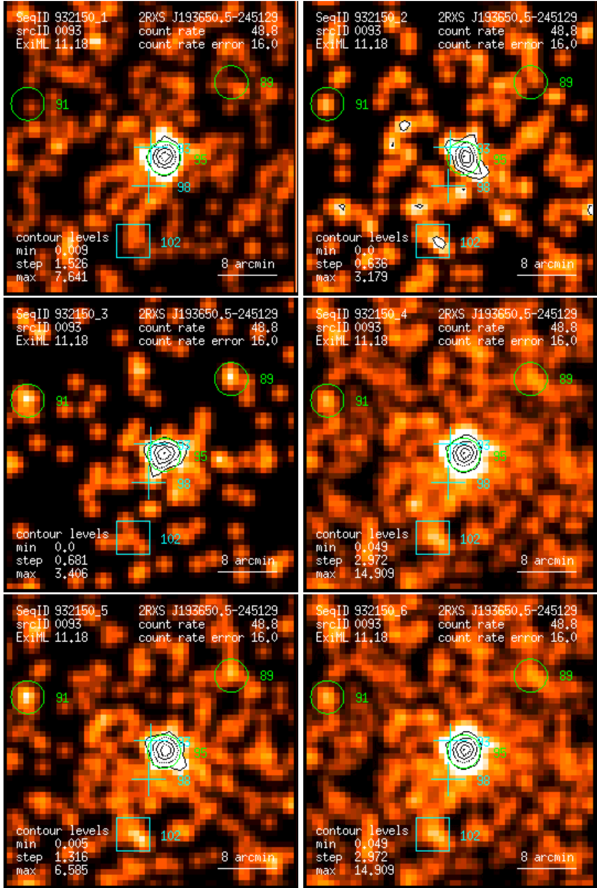
Figure 93: RASS 932150: detection 0093: band rate images, Gaussian filter: (1) PSPC channels 11 – 41, (2) 52 – 90, (3) 91 – 201, (4) 11 – 235, (5) 52 – 201, (6) 11 – 201. Broad band rates in counts/ks. Band rate contour levels in counts/ks/arcmin 2 .
