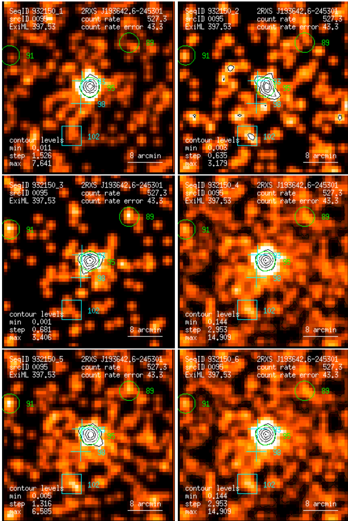
Figure 95: RASS 932150: detection 0095: band rate images, Gaussian filter: (1) PSPC channels 11 – 41, (2) 52 – 90, (3) 91 – 201, (4) 11 – 235, (5) 52 – 201, (6) 11 – 201. Broad band rates in counts/ks. Band rate contour levels in counts/ks/arcmin 2 .
