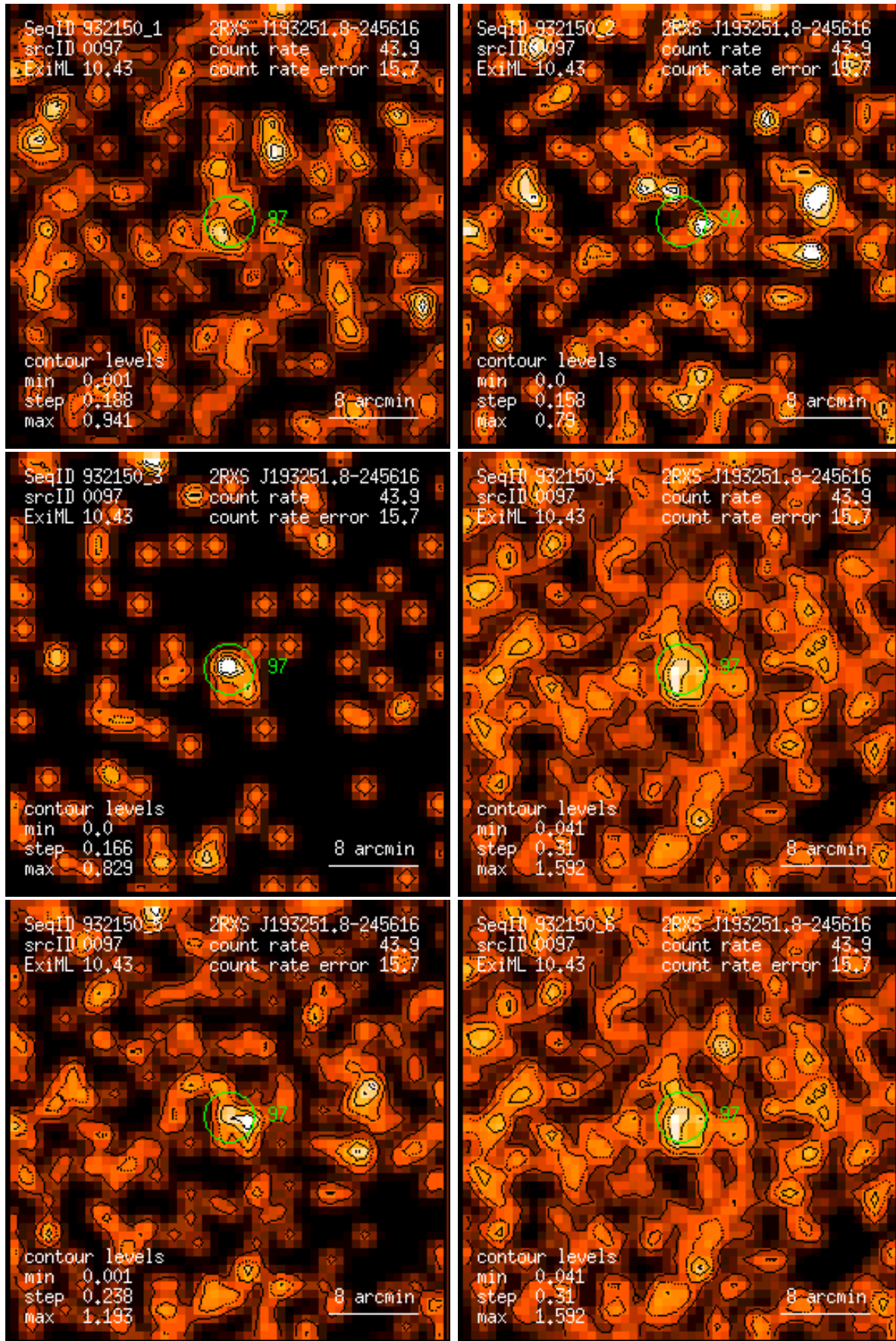
Figure 97: RASS 932150: detection 0097: band rate images, Gaussian filter: (1) PSPC channels 11 – 41, (2) 52 – 90, (3) 91 – 201, (4) 11 – 235, (5) 52 – 201, (6) 11 – 201. Broad band rates in counts/ks. Band rate contour levels in counts/ks/arcmin 2 .
