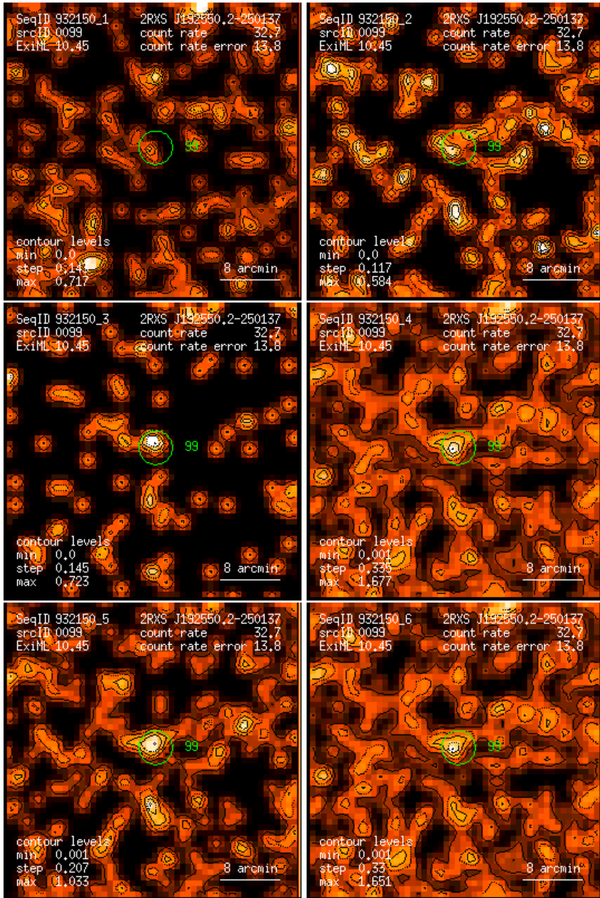
Figure 99: RASS 932150: detection 0099: band rate images, Gaussian filter: (1) PSPC channels 11 – 41, (2) 52 – 90, (3) 91 – 201, (4) 11 – 235, (5) 52 – 201, (6) 11 – 201. Broad band rates in counts/ks. Band rate contour levels in counts/ks/arcmin 2 .
