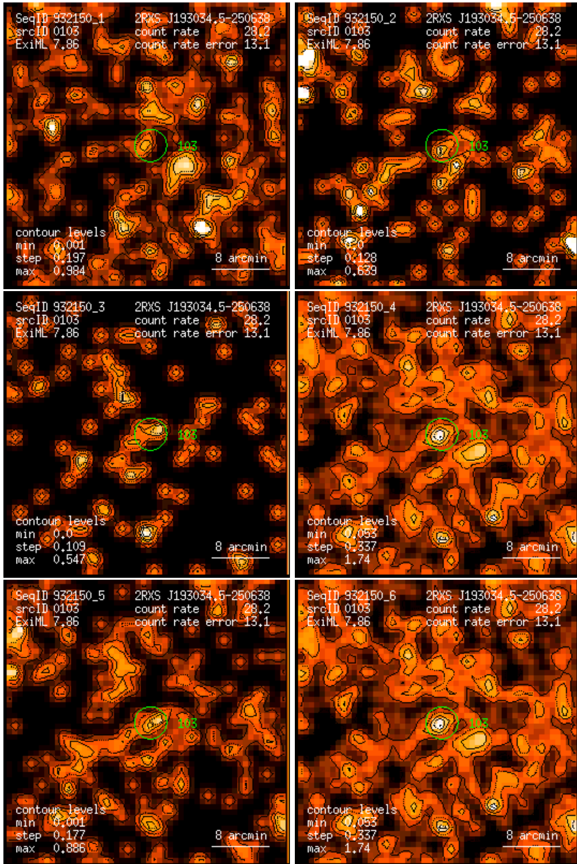
Figure 103: RASS 932150: detection 0103: band rate images, Gaussian filter: (1) PSPC channels 11 – 41, (2) 52 – 90, (3) 91 – 201, (4) 11 – 235, (5) 52 – 201, (6) 11 – 201. Broad band rates in counts/ks. Band rate contour levels in counts/ks/arcmin 2 .
