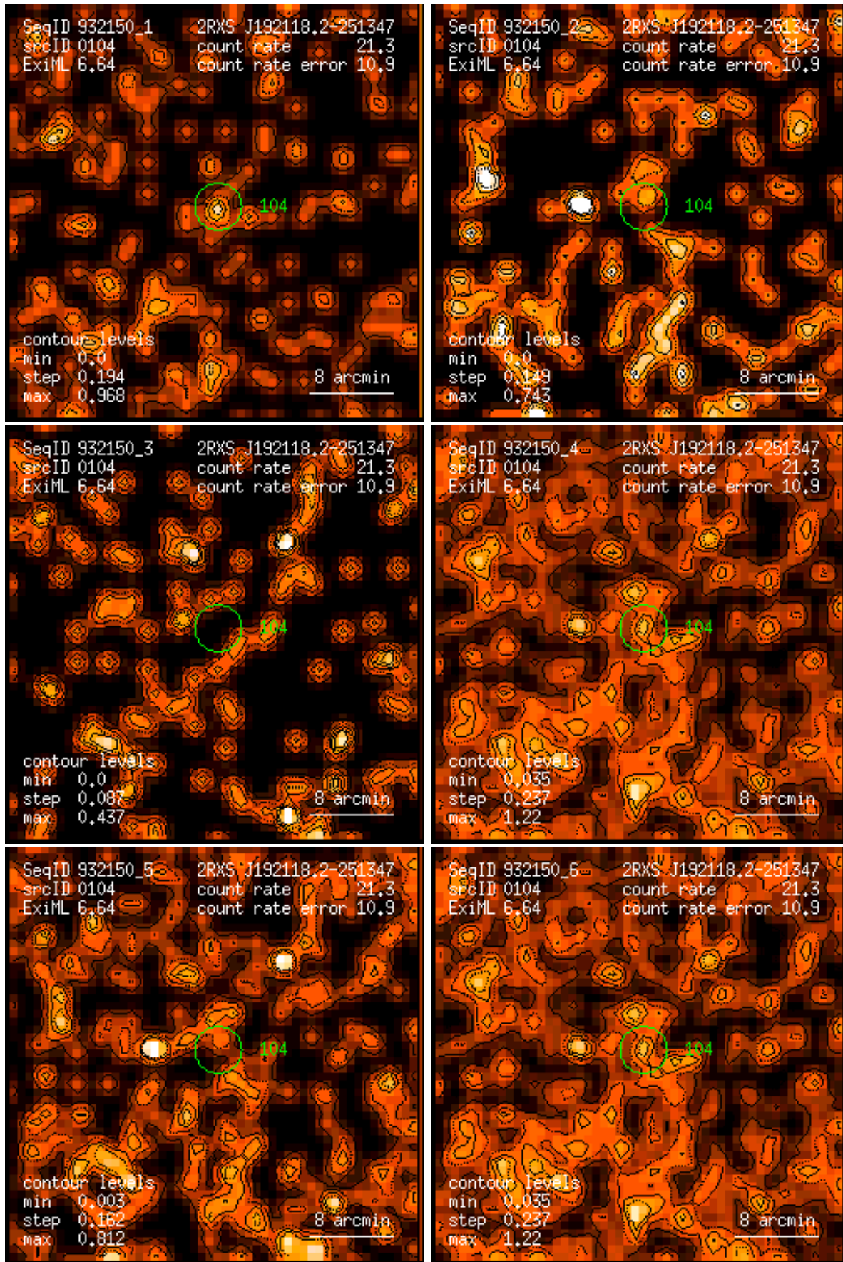
Figure 104: RASS 932150: detection 0104: band rate images, Gaussian filter: (1) PSPC channels 11 – 41, (2) 52 – 90, (3) 91 – 201, (4) 11 – 235, (5) 52 – 201, (6) 11 – 201. Broad band rates in counts/ks. Band rate contour levels in counts/ks/arcmin 2 .
