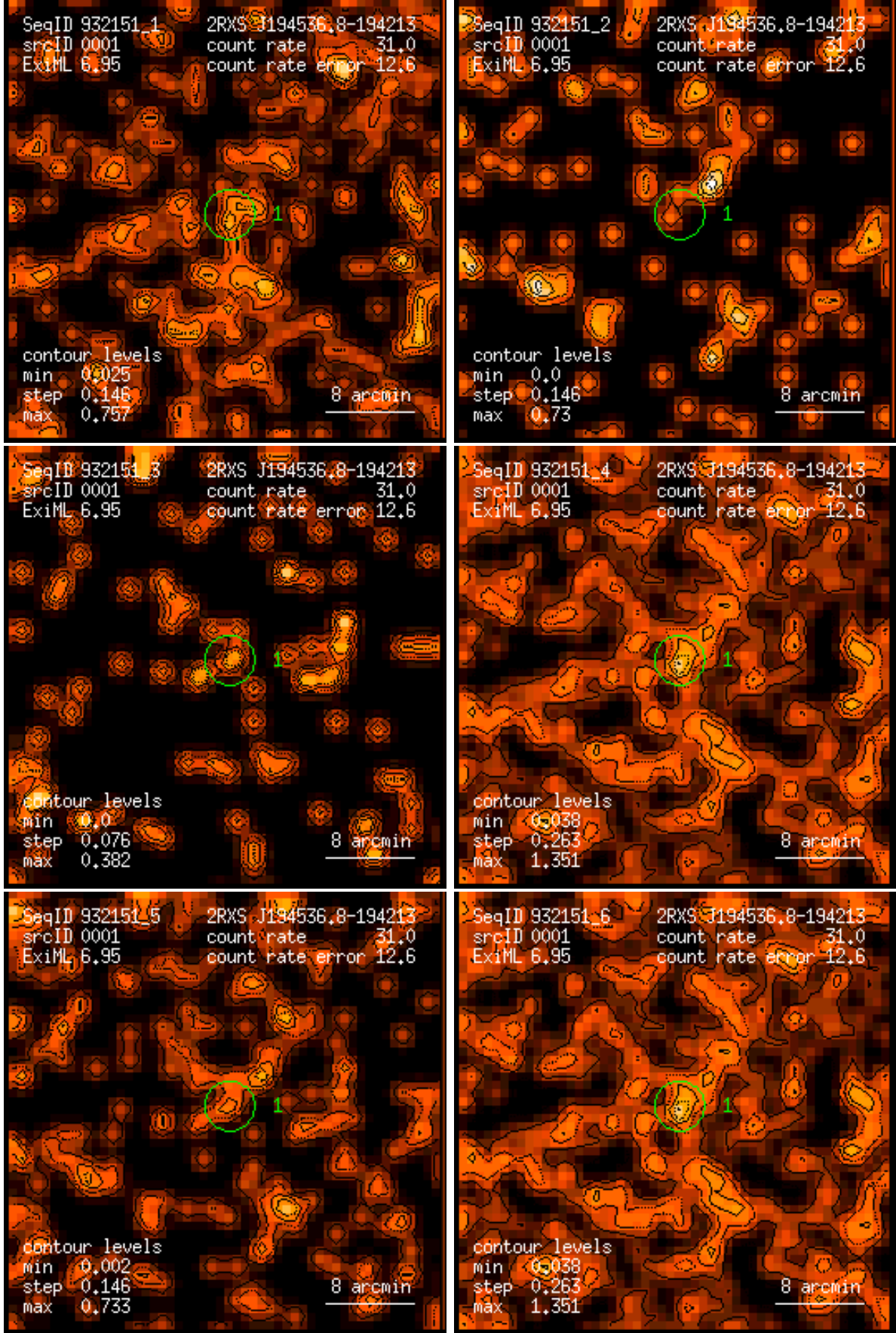
Figure 1: RASS 932151: detection 0001: band rate images, Gaussian filter: (1) PSPC channels 11 – 41, (2) 52 – 90, (3) 91 – 201, (4) 11 – 235, (5) 52 – 201, (6) 11 – 201. Broad band rates in counts/ks. Band rate contour levels in counts/ks/arcmin 2 .
