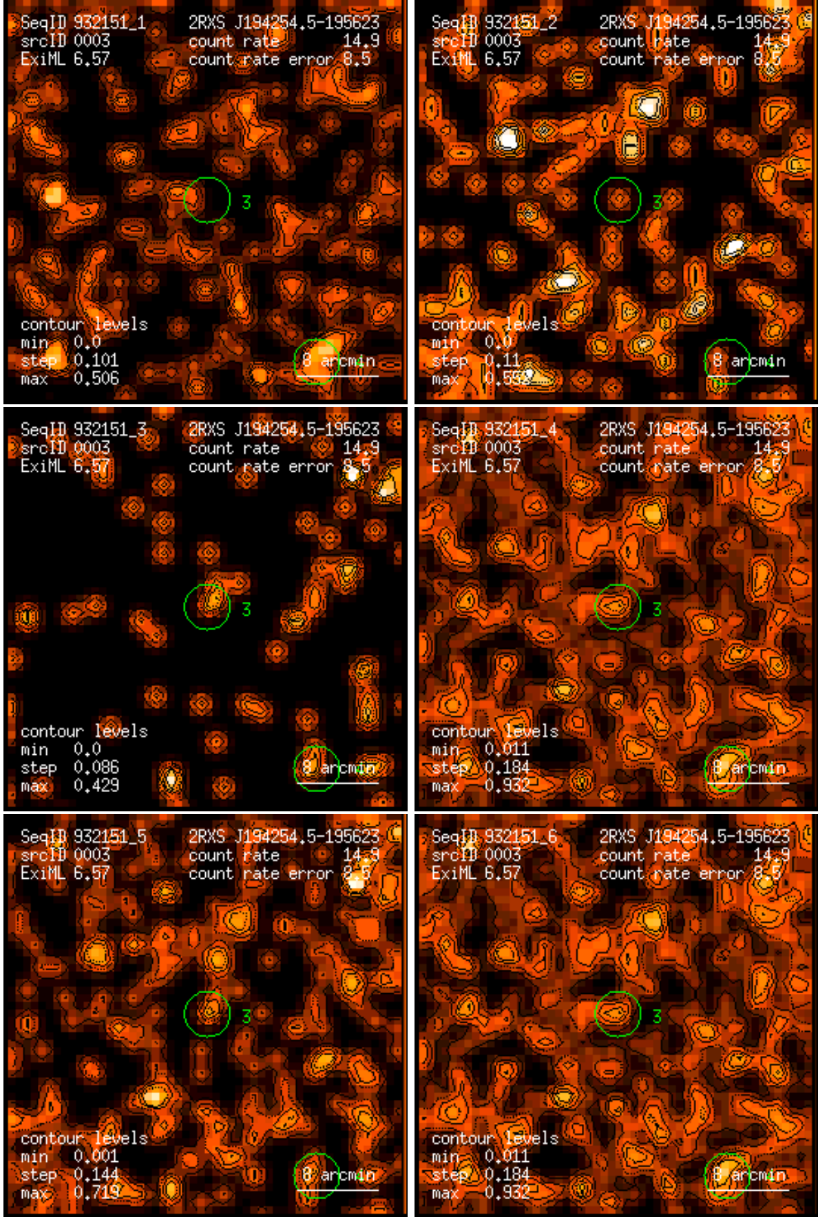
Figure 3: RASS 932151: detection 0003: band rate images, Gaussian filter: (1) PSPC channels 11 – 41, (2) 52 – 90, (3) 91 – 201, (4) 11 – 235, (5) 52 – 201, (6) 11 – 201. Broad band rates in counts/ks. Band rate contour levels in counts/ks/arcmin 2 .
