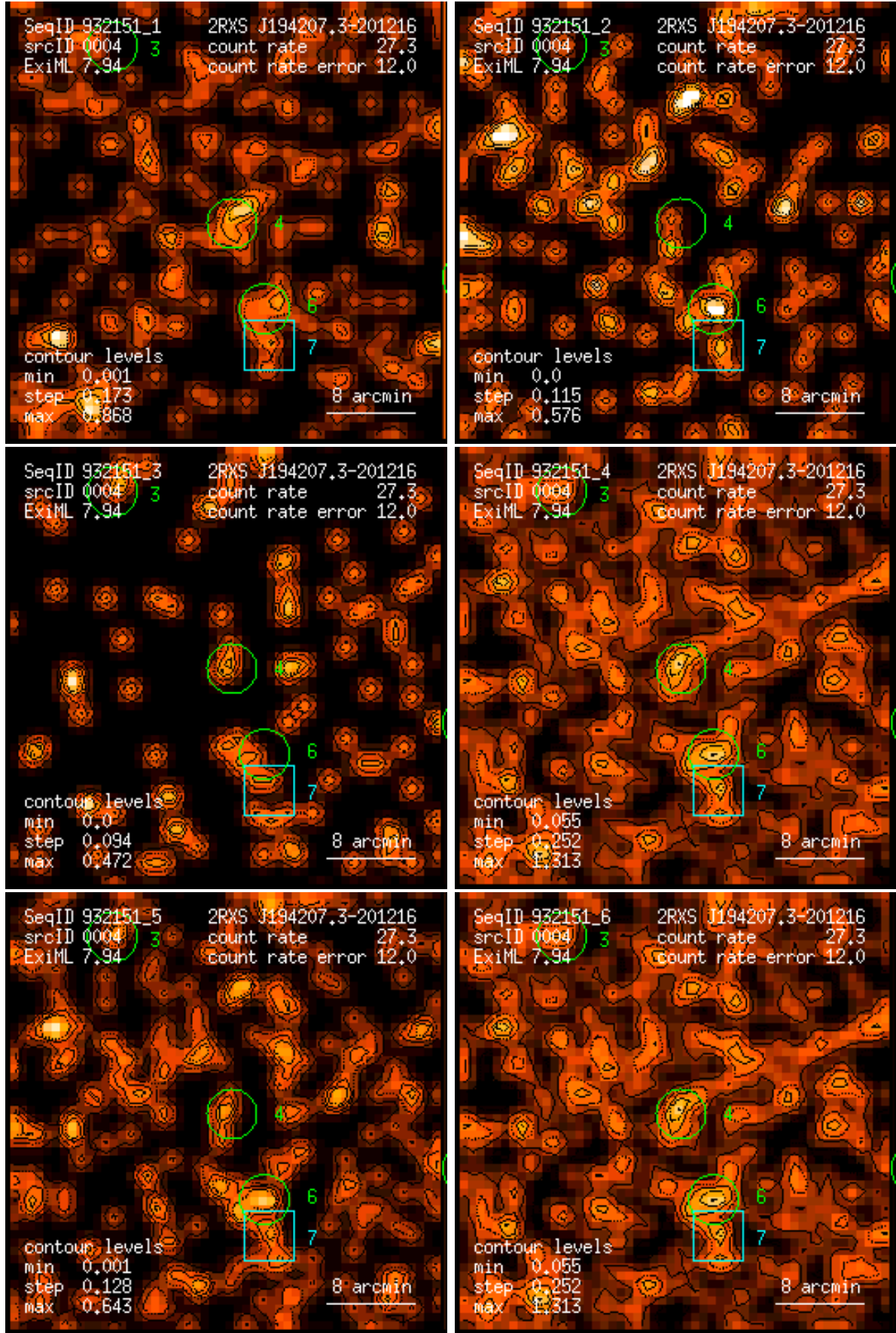
Figure 4: RASS 932151: detection 0004: band rate images, Gaussian filter: (1) PSPC channels 11 – 41, (2) 52 – 90, (3) 91 – 201, (4) 11 – 235, (5) 52 – 201, (6) 11 – 201. Broad band rates in counts/ks. Band rate contour levels in counts/ks/arcmin 2 .
