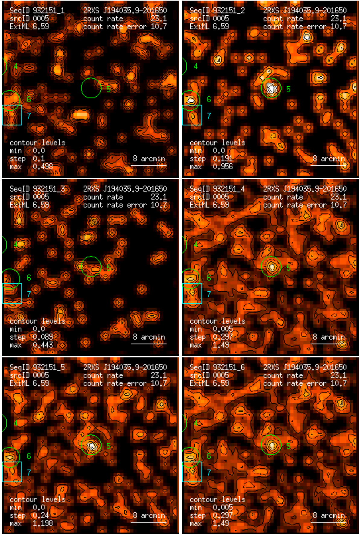
Figure 5: RASS 932151: detection 0005: band rate images, Gaussian filter: (1) PSPC channels 11 – 41, (2) 52 – 90, (3) 91 – 201, (4) 11 – 235, (5) 52 – 201, (6) 11 – 201. Broad band rates in counts/ks. Band rate contour levels in counts/ks/arcmin 2 .
