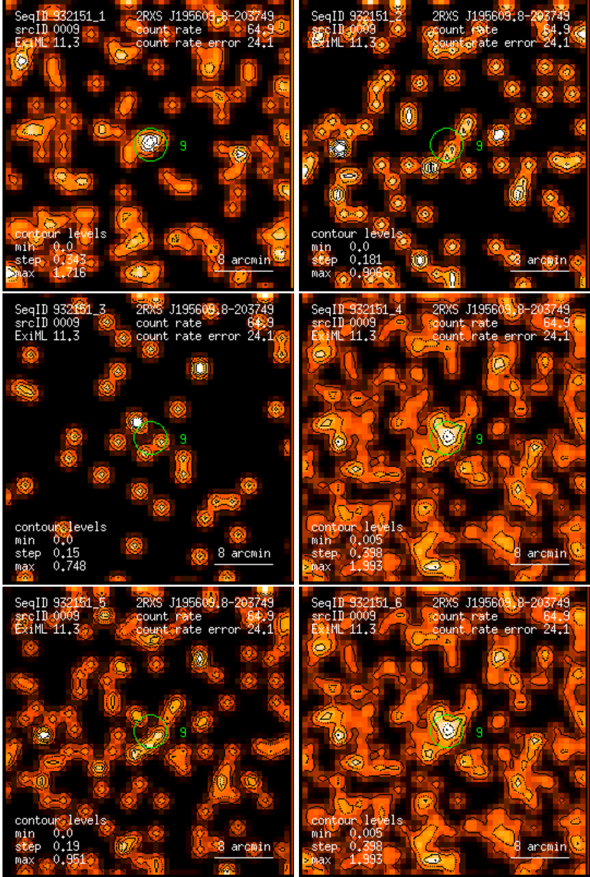
Figure 9: RASS 932151: detection 0009: band rate images, Gaussian filter: (1) PSPC channels 11 – 41, (2) 52 – 90, (3) 91 – 201, (4) 11 – 235, (5) 52 – 201, (6) 11 – 201. Broad band rates in counts/ks. Band rate contour levels in counts/ks/arcmin 2 .
