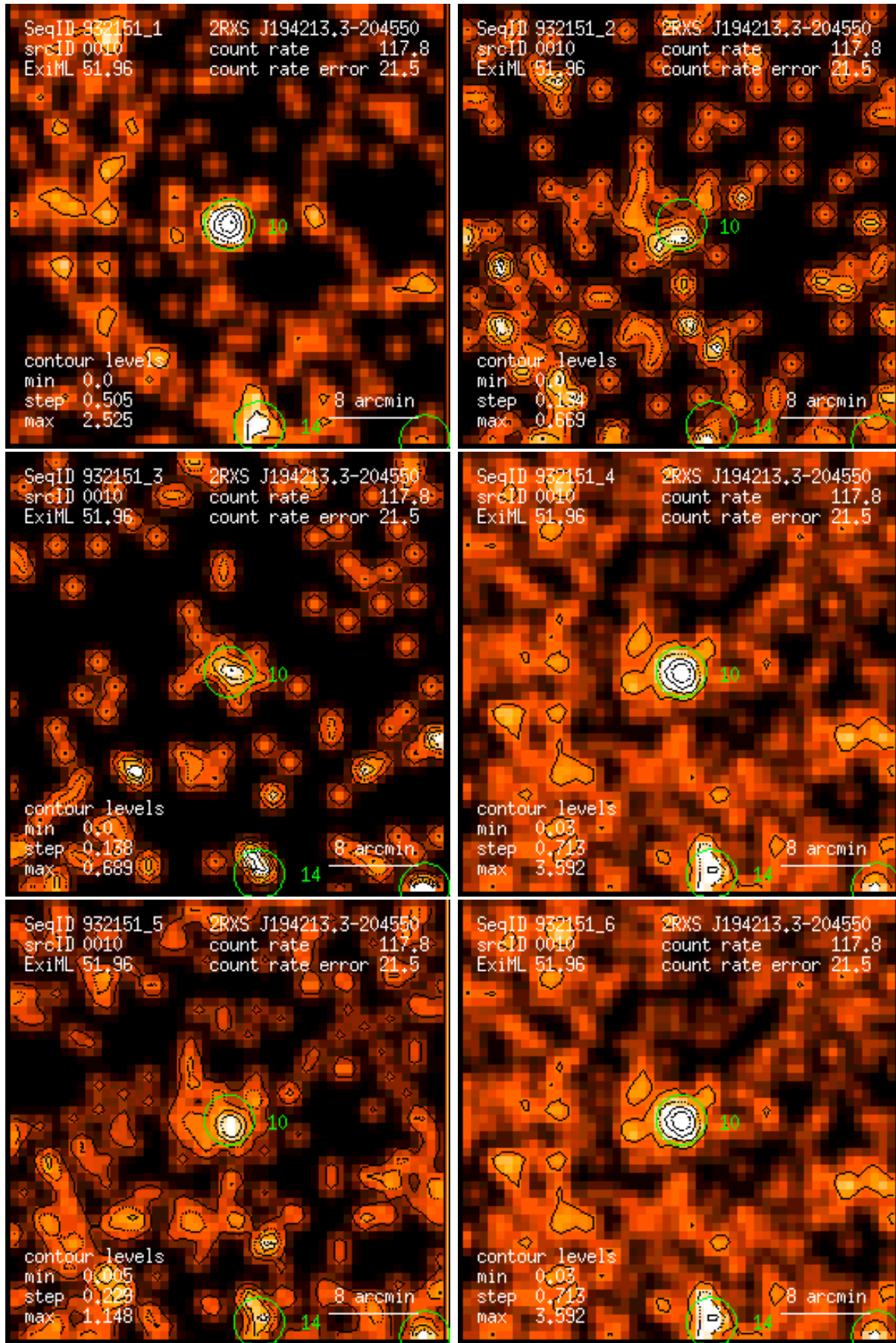
Figure 10: RASS 932151: detection 0010: band rate images, Gaussian filter: (1) PSPC channels 11 – 41, (2) 52 – 90, (3) 91 – 201, (4) 11 – 235, (5) 52 – 201, (6) 11 – 201. Broad band rates in counts/ks. Band rate contour levels in counts/ks/arcmin 2 .
