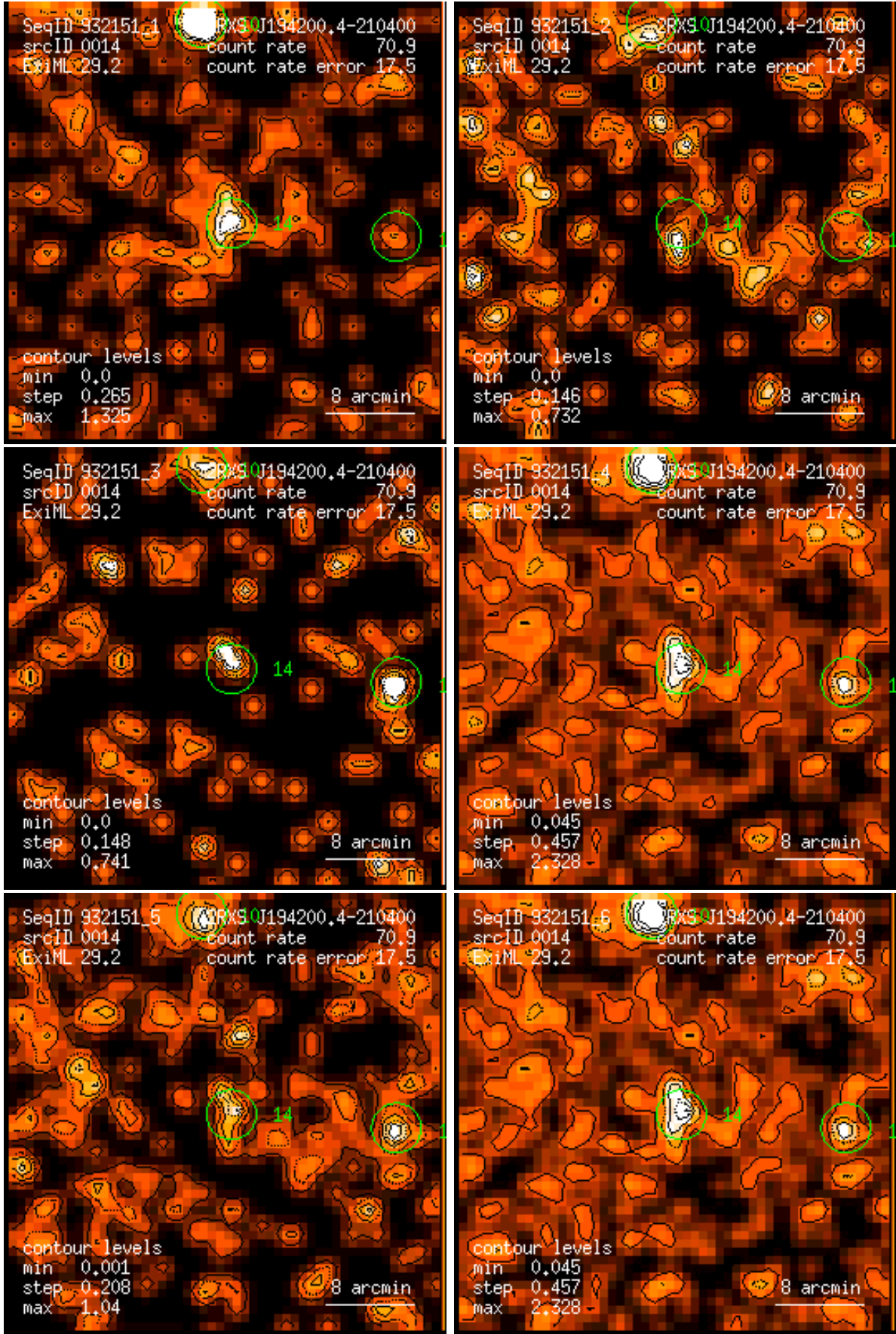
Figure 14: RASS 932151: detection 0014: band rate images, Gaussian filter: (1) PSPC channels 11 – 41, (2) 52 – 90, (3) 91 – 201, (4) 11 – 235, (5) 52 – 201, (6) 11 – 201. Broad band rates in counts/ks. Band rate contour levels in counts/ks/arcmin 2 .
