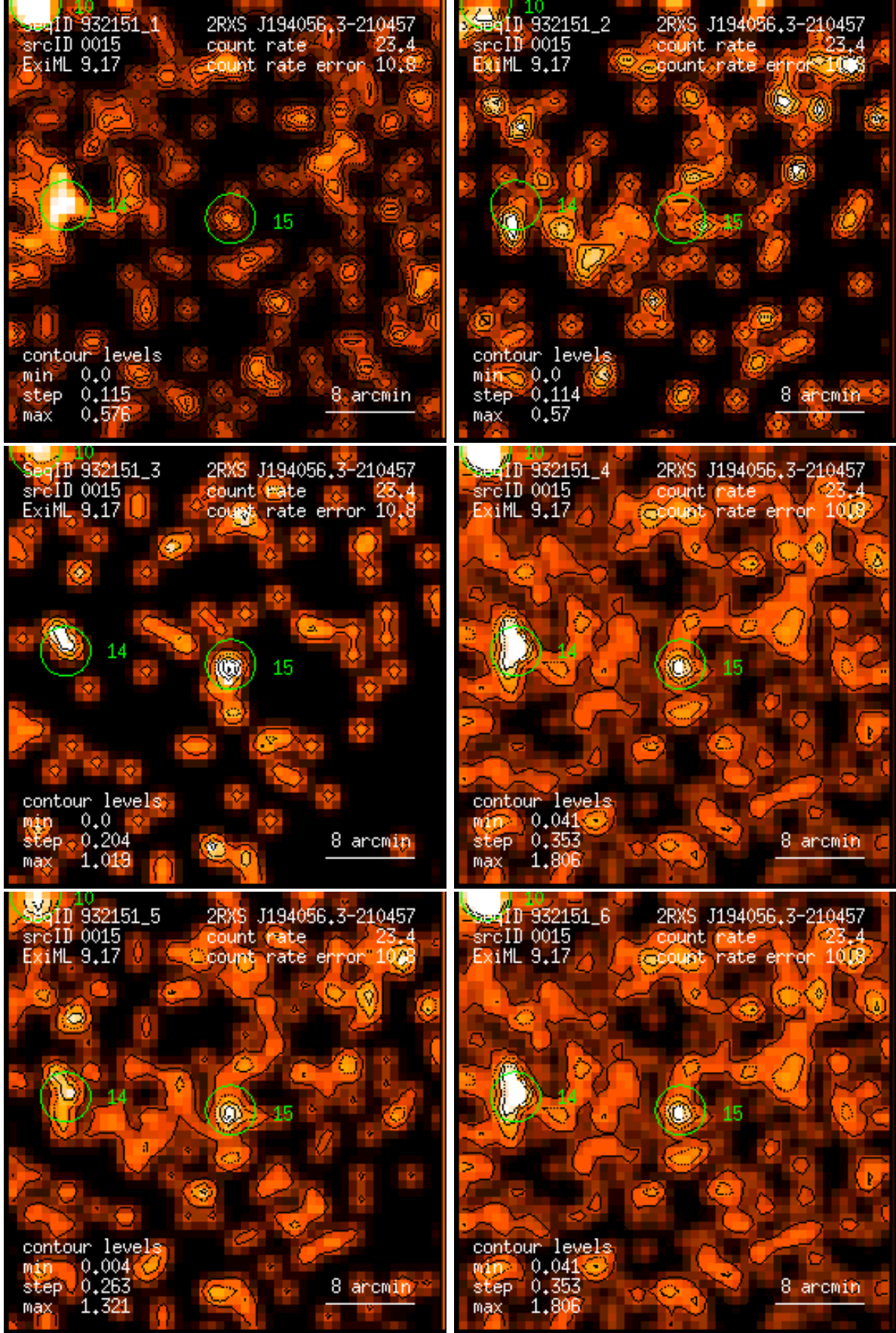
Figure 15: RASS 932151: detection 0015: band rate images, Gaussian filter: (1) PSPC channels 11 – 41, (2) 52 – 90, (3) 91 – 201, (4) 11 – 235, (5) 52 – 201, (6) 11 – 201. Broad band rates in counts/ks. Band rate contour levels in counts/ks/arcmin 2 .
