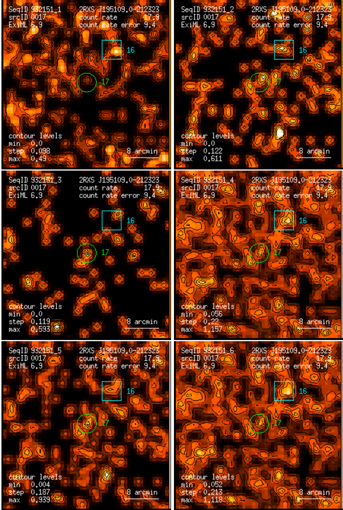
Figure 17: RASS 932151: detection 0017: band rate images, Gaussian filter: (1) PSPC channels 11 – 41, (2) 52 – 90, (3) 91 – 201, (4) 11 – 235, (5) 52 – 201, (6) 11 – 201. Broad band rates in counts/ks. Band rate contour levels in counts/ks/arcmin 2 .
