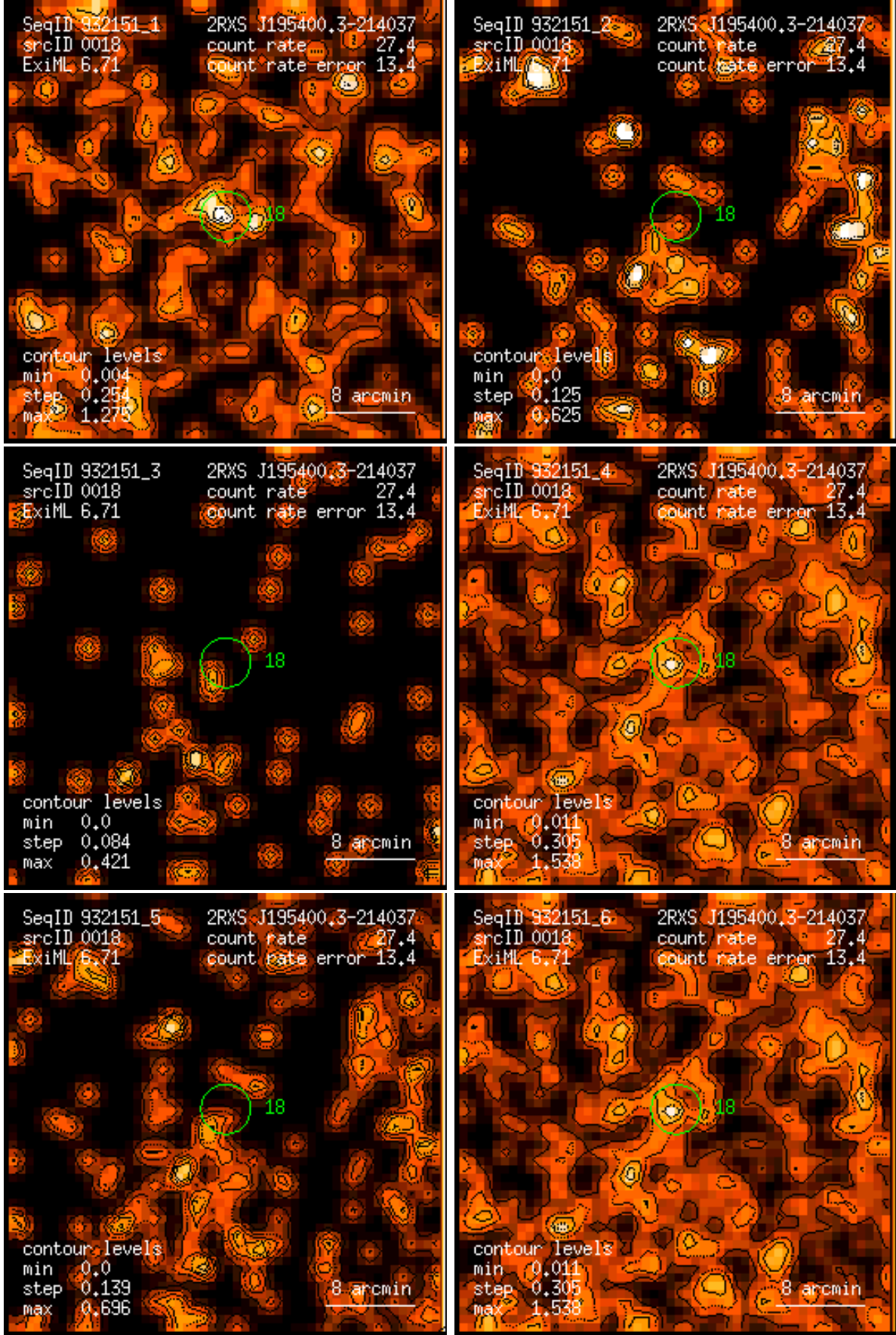
Figure 18: RASS 932151: detection 0018: band rate images, Gaussian filter: (1) PSPC channels 11 – 41, (2) 52 – 90, (3) 91 – 201, (4) 11 – 235, (5) 52 – 201, (6) 11 – 201. Broad band rates in counts/ks. Band rate contour levels in counts/ks/arcmin 2 .
