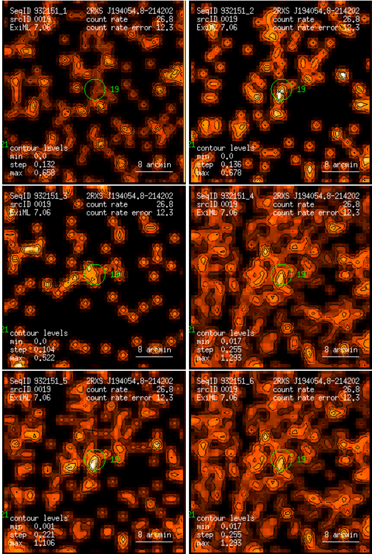
Figure 19: RASS 932151: detection 0019: band rate images, Gaussian filter: (1) PSPC channels 11 – 41, (2) 52 – 90, (3) 91 – 201, (4) 11 – 235, (5) 52 – 201, (6) 11 – 201. Broad band rates in counts/ks. Band rate contour levels in counts/ks/arcmin 2 .
