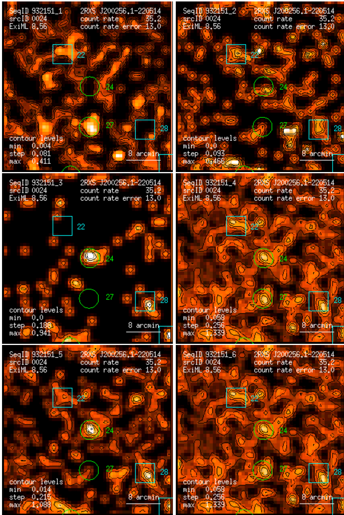
Figure 24: RASS 932151: detection 0024: band rate images, Gaussian filter: (1) PSPC channels 11 – 41, (2) 52 – 90, (3) 91 – 201, (4) 11 – 235, (5) 52 – 201, (6) 11 – 201. Broad band rates in counts/ks. Band rate contour levels in counts/ks/arcmin 2 .
