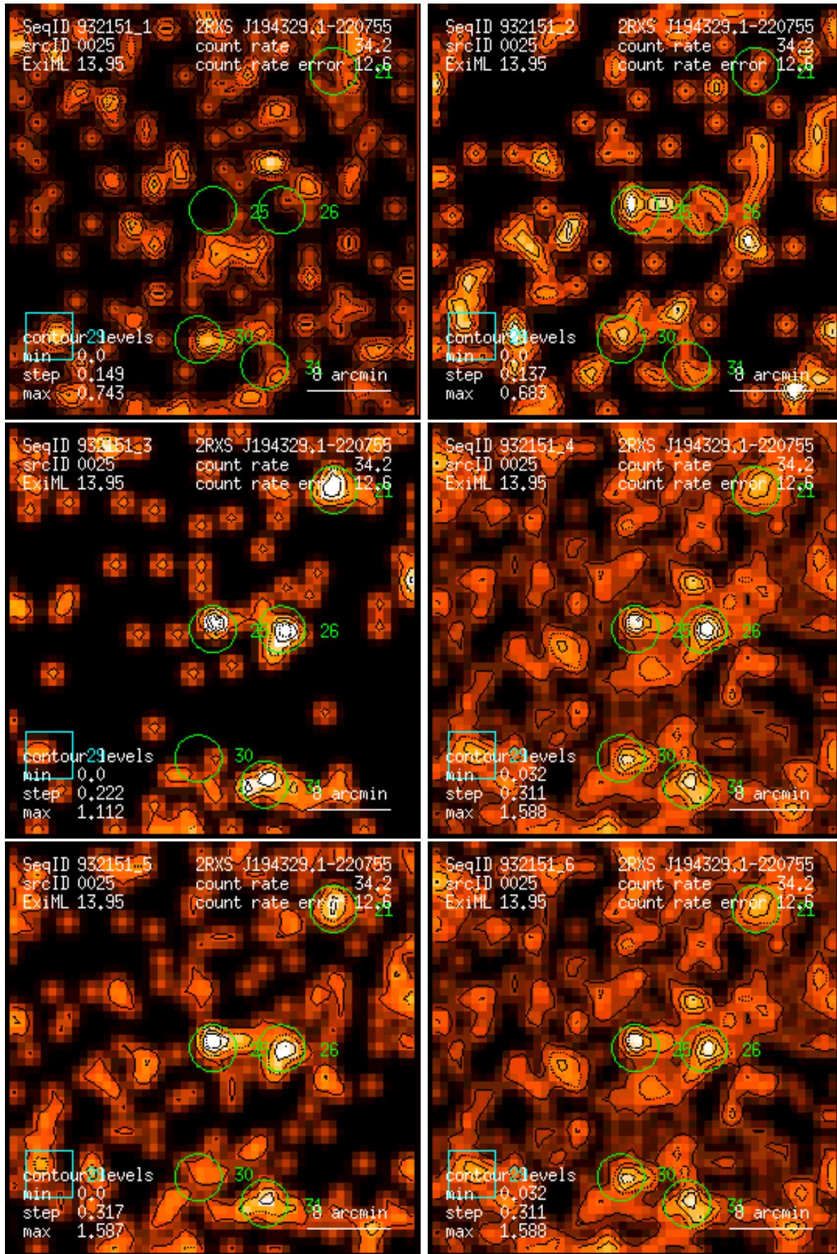
Figure 25: RASS 932151: detection 0025: band rate images, Gaussian filter: (1) PSPC channels 11 – 41, (2) 52 – 90, (3) 91 – 201, (4) 11 – 235, (5) 52 – 201, (6) 11 – 201. Broad band rates in counts/ks. Band rate contour levels in counts/ks/arcmin 2 .
