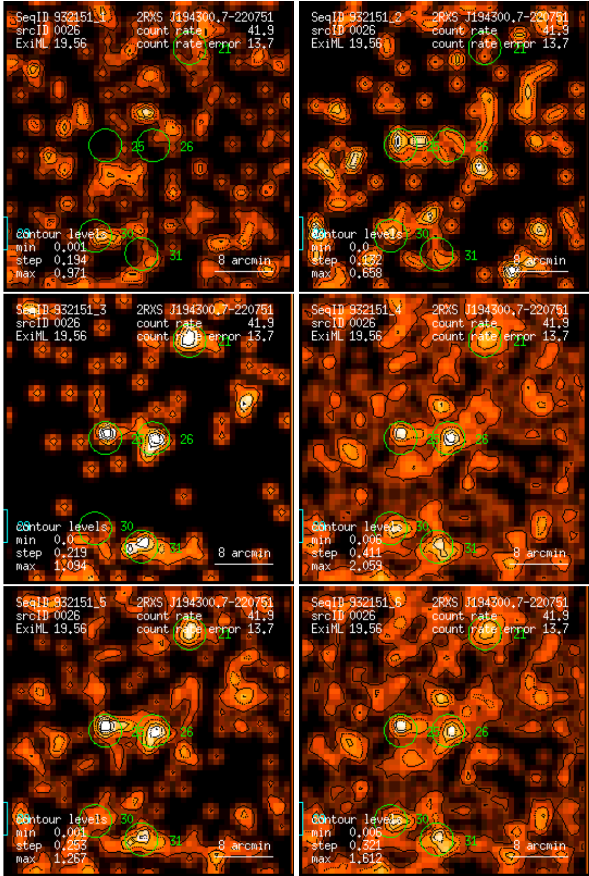
Figure 26: RASS 932151: detection 0026: band rate images, Gaussian filter: (1) PSPC channels 11 – 41, (2) 52 – 90, (3) 91 – 201, (4) 11 – 235, (5) 52 – 201, (6) 11 – 201. Broad band rates in counts/ks. Band rate contour levels in counts/ks/arcmin 2 .
